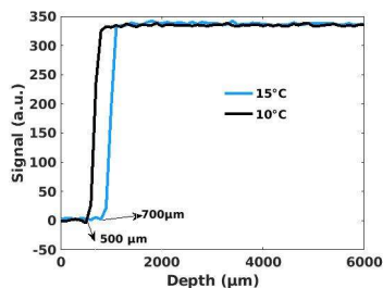
Figure 1: Sample profiles recorded at a magnet temperature of 10 (black) and 15°C (blue). A shift of 200 \mu\text{m} is observed for this 5°C difference.
