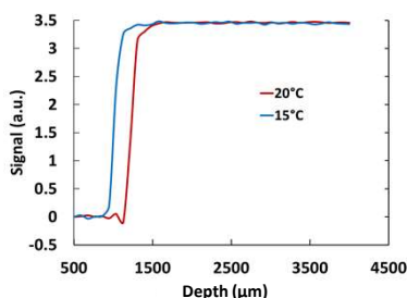
Figure 2: Sample profiles recorded 2 hours after the temperature stabilization of the magnet at 15 (blue) and 20°C (red). A shift of 241 \mu\text{m} is observed.
