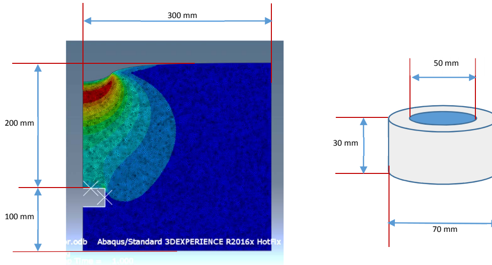
Figure 1: (a) Finite element model of soil-stress transducer interaction and (a) disc-shaped transducer.
