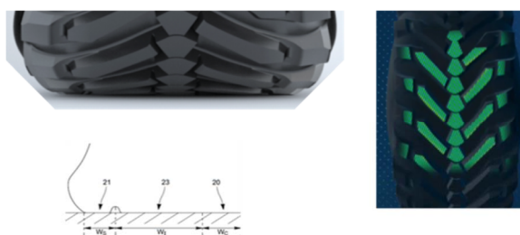
Fig. 4: Tire shape and contact patch in field configuration
