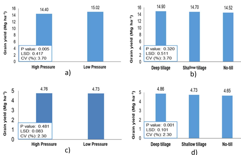
58 Fig. 1. Effect of tire inflation pressure and tillage systems on the grain yields of corn and soybean 59 (Figs. a&b are corn and c&d are soybean, respectively).
