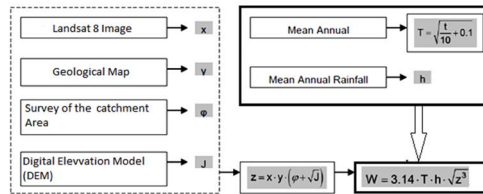
Figure2: EPM Flowchart
