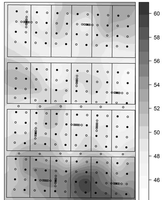
Figure 1. Map of sampling points and SOC stocks (t ha -1 ) in the reference layer (0-35 cm) in 2009 (obtained by ordinary kriging).
