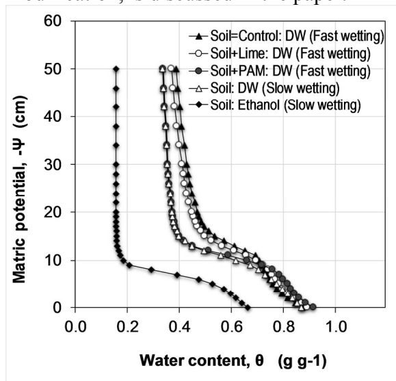
Figure 1. Water retention of clay Luvisols, control, treated with slaked lime ( 1.6 \text{ gL}^{-1} ) and polyacrylamide (PAM= 200 \text{ mgL}^{-1} ), and wetted (fast or slow) with deionized water (DW) or ethanol.
