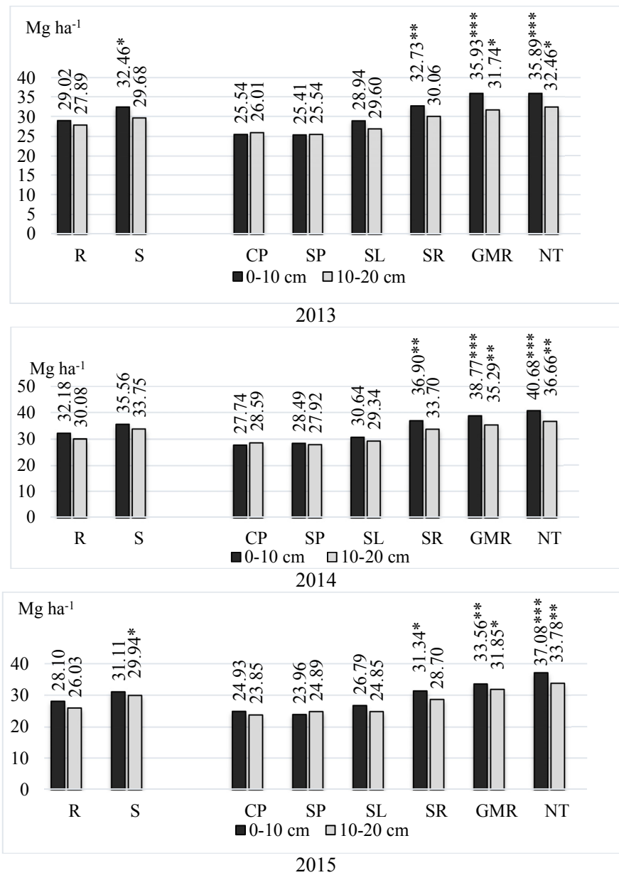
Figure 1. Soil organic carbon stocks in the upper and bottom plough layers,
