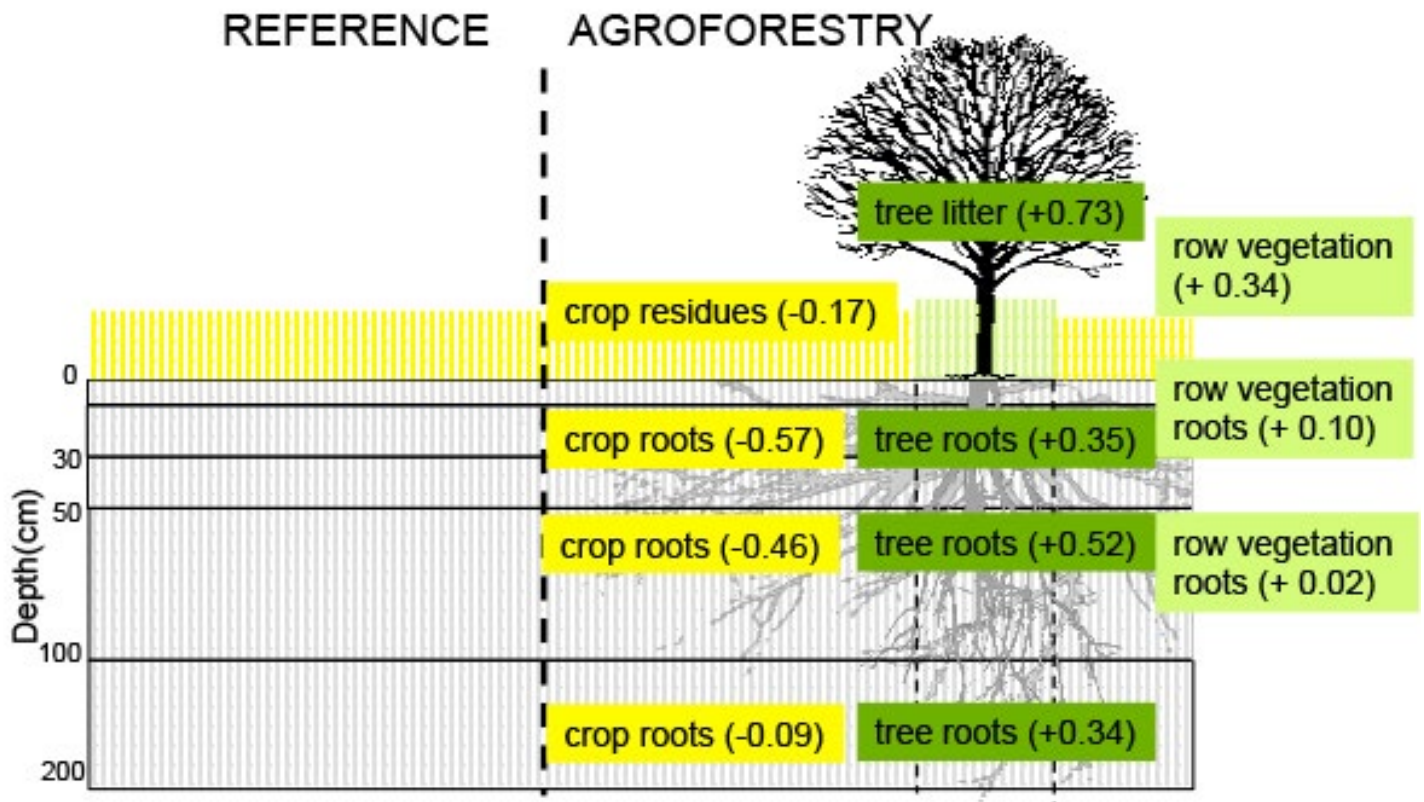
Figure 1. Measured differences in fresh organic carbon inputs from the vegetation to soil in the agroforestry plot at Restinclières, compared to the reference plots. All values are in tC ha -1 yr -1 and only average values are presented here.
