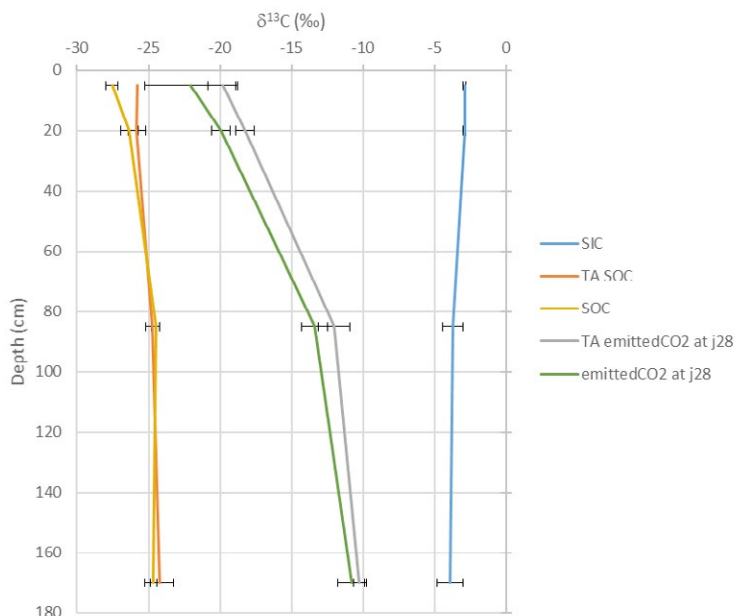
Fig. 1 13 C (‰) profil of SOC and SIC and the CO 2 emitted from 2 soils with similar SIC contents but different SOC contents after 28 days (21-28 days).
