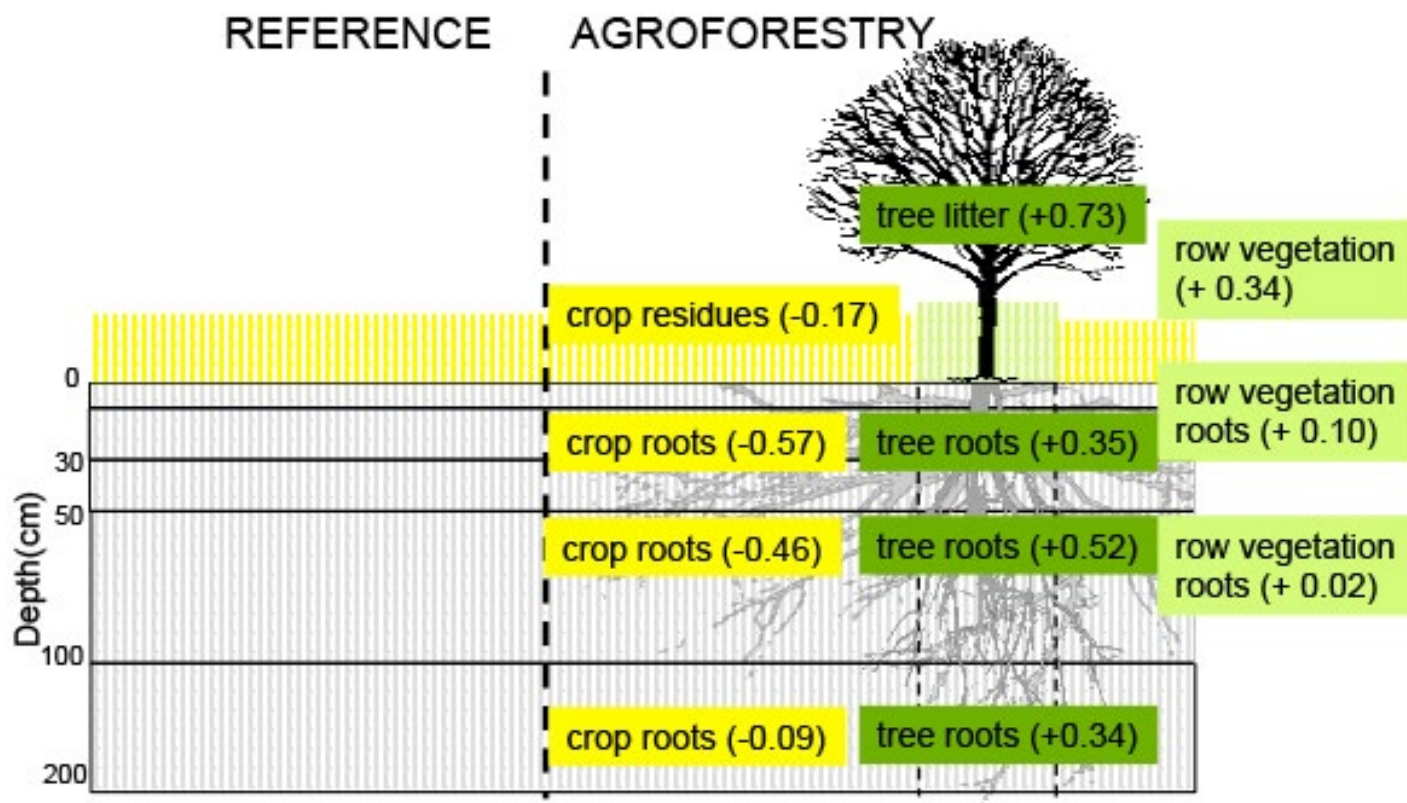
Figure 1. Measured differences in fresh organic carbon inputs from the vegetation to soil in the agroforestry plot at Restinclières, compared to the reference plots. All values are in \text{tC ha}^{-1} \text{yr}^{-1} and only average values are presented here.
