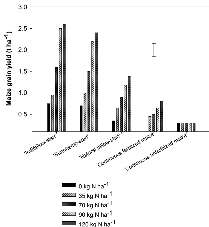
Figure 1. Maize grain yields ( \text{t ha}^{-1} ) and responses to mineral N fertilizer different ISFM sequences on degraded soils in Hwedza farming communities in Zimbabwe. Vertical bars represent standard error of the difference of means (SEDs)
