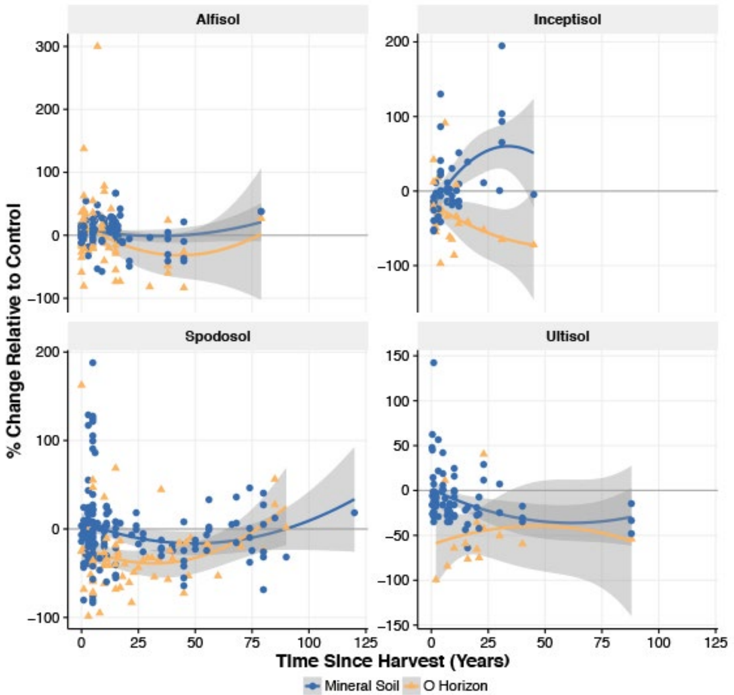
Fig. 2: Temporal patterns in both O horizon (yellow triangles) and mineral soil (blue circles) C pools for Alfisol, Inceptisol, Spodosol, and Ultisol orders. Other orders are not shown due to inadequate sampling over time. Regression lines show trends with time using a second order polynomial ( \text{Time} + \text{Time}^2 ). For the overall model, F=9.205 on 7 and 532 degrees of freedom, \text{Adj. } R^2 = 0.1 , p < 0.0001 . Reproduced from (James and Harrison, 2016).
