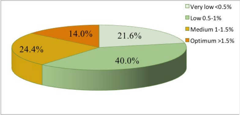
Figure 1. Range of organic carbon content in agricultural soils of Iran
