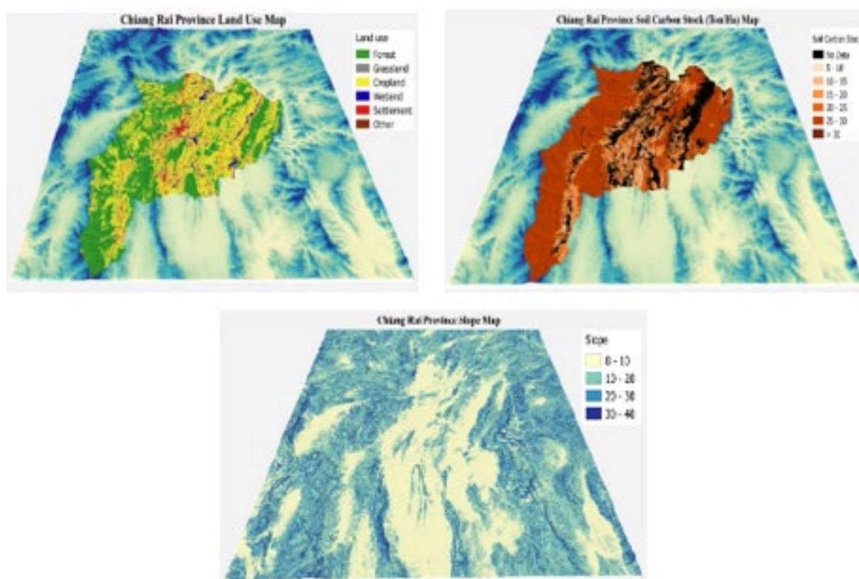
Fig. 1: Chaing Rai Province (a) Land use (b) Soil carbon stock (c) Slope map
