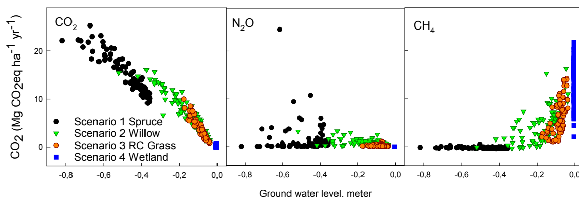
Fig. 2: Annual mean soil flux of \text{CO}_2 due to peat decomposition, \text{N}_2\text{O} and \text{CH}_4 for the four scenarios with 1) spruce, 2) willow, 3) reed canary grass and 4) wetland mosses, related to annual mean groundwater level over 80 years.
