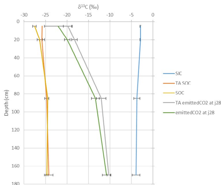
Fig. 1 13 C (‰) profile of SOC and SIC and the CO 2 emitted from 2 soils with similar SIC contents but different SOC contents after 28 days (21-28 days).
