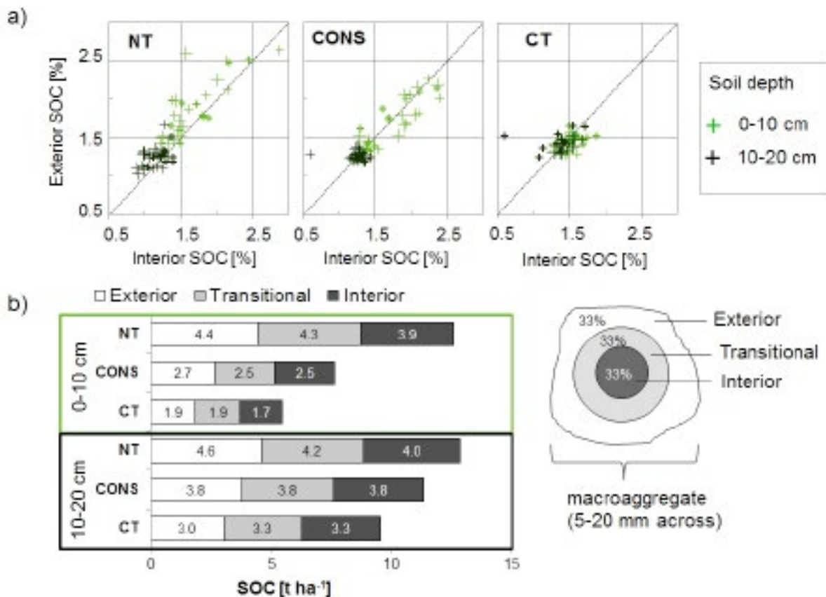
Fig. 1: Relation between exterior and interior SOC within macroaggregates (5–20 mm across) from 0–10 and 10–20 cm sampling depth of a sandy-loam Stagnic Luvisol (published in Mordhorst, 2013) (a) and calculated mean SOC stocks of concentric aggregate layers (b) depending on tillage intensity (CT = conventional ploughing, CONS = Reduced tillage (harrowing 8–10 cm), NT = No-tillage).
