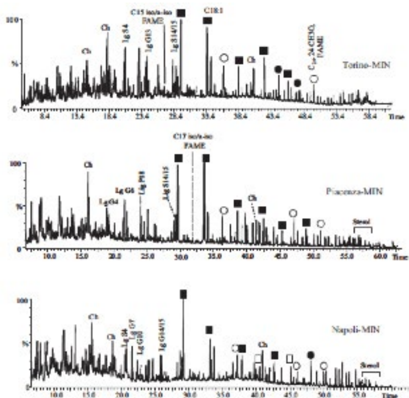
Figure 2 Representative total ion chromatograms of thermochemolysis products released from soil samples (●) alcohol; Ch, carbohydrate; (□) alkyl-dioic acid DIME; (■) FAME; (○) hydroxy-FAME; Lg, lignin.
