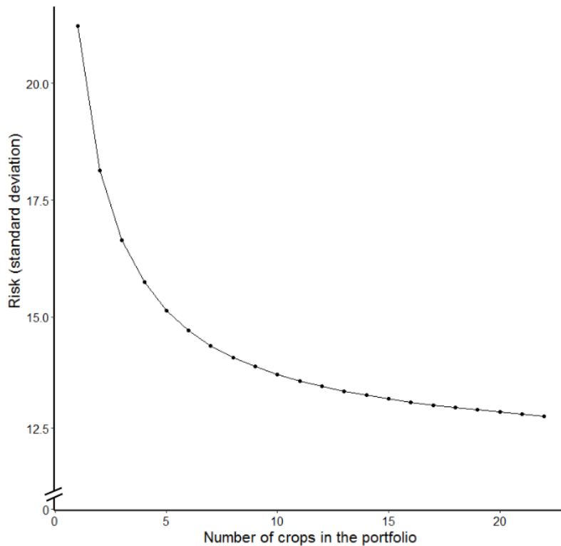
Figure 5. Effect of increasing portfolio compositions from 1 to 22 crops on the portfolio’s standard deviation.
