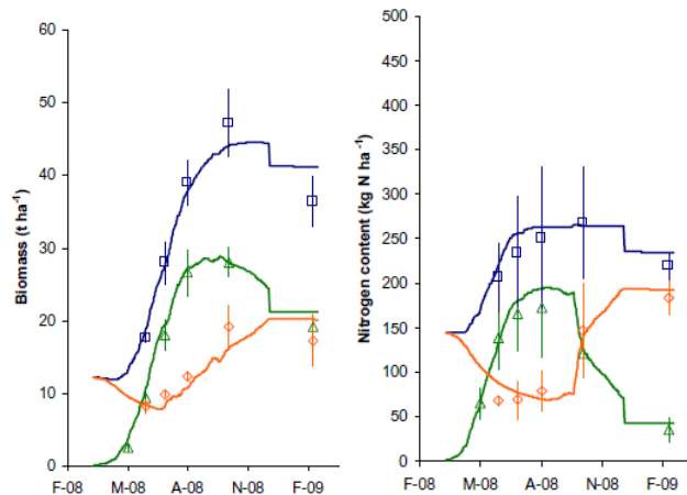
Figure 1: Simulation of biomass and nitrogen fluxes in perennial organs (orange), aboveground organs (green) and aboveground + perennial organs (blue) of Miscanthus.
