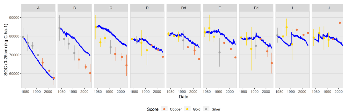
Figure 1. Comparison of simulated (blue lines) and observed (points) SOC dynamics over 27 years at Kerbernez site for nine crop-grassland rotations.
