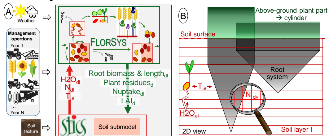
Figure 3. Connecting the STICS soil submodel to the 3D individual-based FLORSYS weed dynamics model. A. Each day d , STICS provides water potential, nitrogen availability and temperature for each soil layer I . These drive seed and plant processes in FLORSYS, together with weather and cropping-system inputs. FLORSYS returns canopy information to STICS to calculate soil variables for the next day. B. In FLORSYS, soil temperature and water potential drive seed germination and pre-emergent growth, soil temperature drives root-system growth. Available nitrogen is distributed inside soil voxels (3D pixels) in each soil layer and extracted by the roots inside each voxel.
