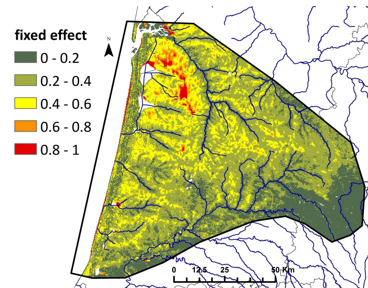
Fig. 6: fixed effect
