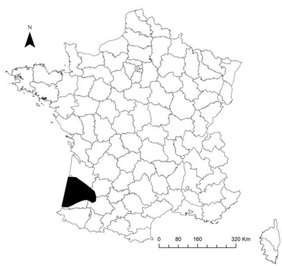
Fig. 1: Study area in 'Landes de Gascogne' (France)
