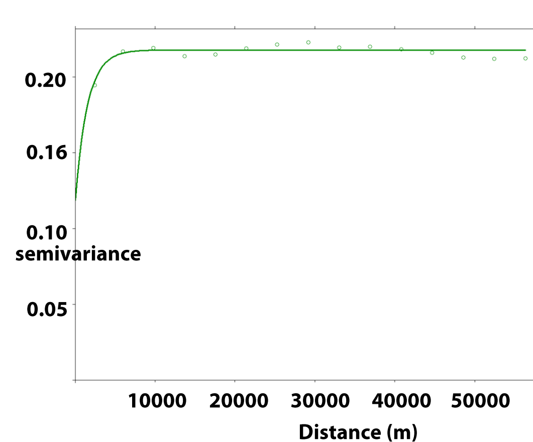
Fig. 5: variogram modelling
