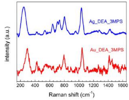
SERS spectra of functionalized MNPs.
