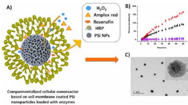
Figure 1. A) Schematic representation of the biomimetic compartmentalized nanoreactor based on the cancer cell membrane coated PSi NPs loaded with HRP enzymes. B) Enzyme activity of nanoreactors analyzed using amplex-red fluorescence assay, compared with different controls. C) Transmission electron micrograph of the compartmentalized cellular nanoreactors.
