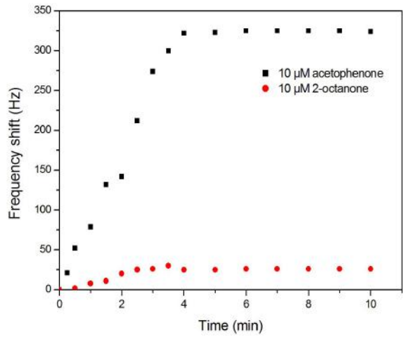
Typical response of 6His-M71 based micro-cantilever
