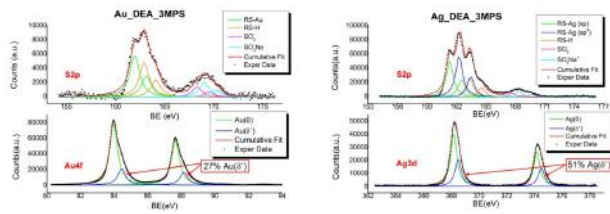
SR-XPS spectra of 2p and metal (Au4f, Ag3d) core levels for gold and silver nanoparticles functionalized by DEA and 3MPS.
