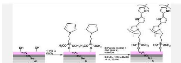
Scheme 1. Schematic representation of: (a) activated Si 3 N 4 , (b) Si 3 N 4 -SPy, and (c) the development of Si 3 N 4 -P(SP 3 -Py) compound materials.
