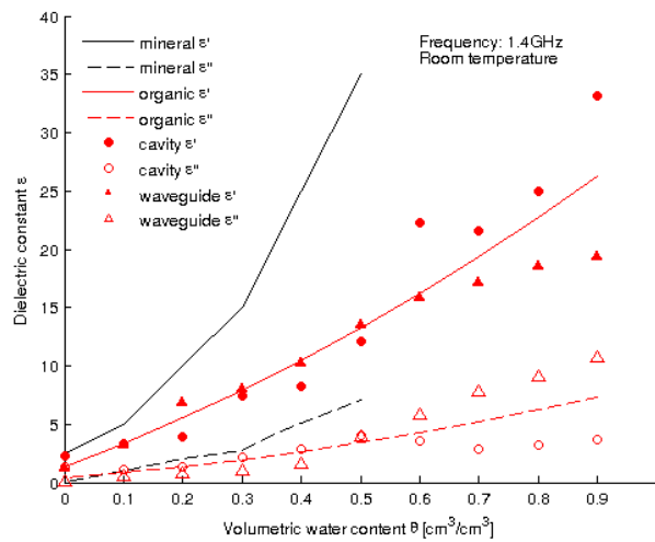
Figure 3: L-band dielectric constants ( \epsilon'/\epsilon'' ), for an average mineral soil (Hallikainen et al., 1985) and fitted through preliminary wave-guide and cavity measurements of organic soil from the Sodankylä forest site.
