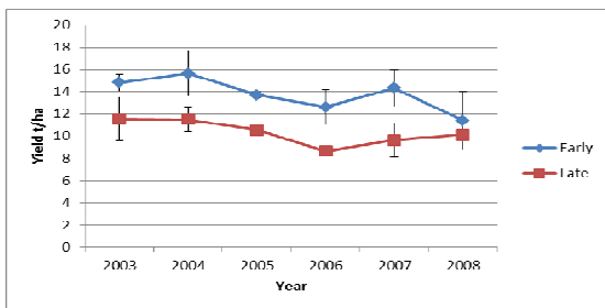
Figure 11: RRES. The annual yield of switchgrass ( cv Cave-in-rock) cut at different harvest dates with 75kg N ha.
