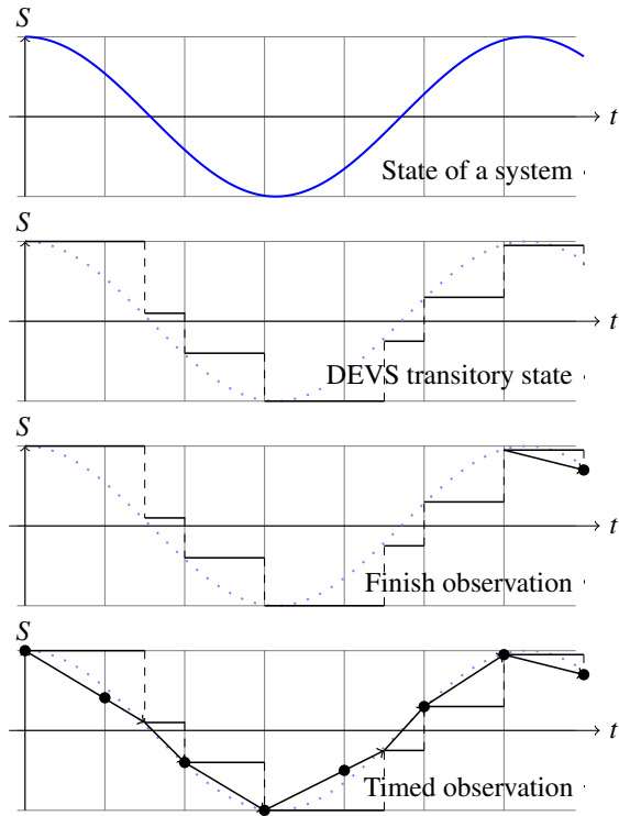
Figure 4: The first figure shows the evolution of the state S of a system over time t . The second figure shows the model of this system in DEVS. This figure shows the trajectory of the state of the DEVS model. The last two figures show the extension observation described in this paper in time-step ( \Delta_t = 1 ) or in finish mode. This extension allows the modeler to provide a function ( observation ) that computes an observation value. Dots are observation values. These values are computed by interpolation of the current DEVS state of s and e , the elapsed time since the last transition.
