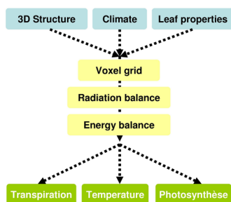
Fig. 1. Main features of the RATP model. The blue boxes are the input data, the main computation processes are in the yellow boxes and the outputs are in the green boxes. Each calculation step is done for each voxel at a 30-min time-step.
