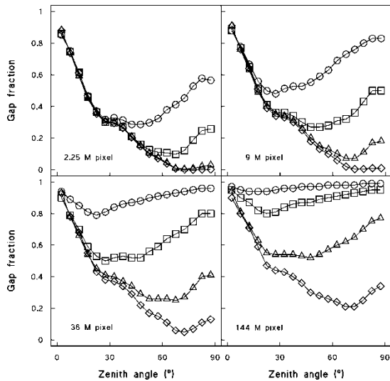
Fig. 4. Estimated gap fraction values in each 5° zenith band from hemispherical images (2.25, 9, 36 or 144 M pixel) generated by the equiangular transform projection procedures of the x, y, z coordinate TLS data for position #1. Same symbols as in Fig. 1.
