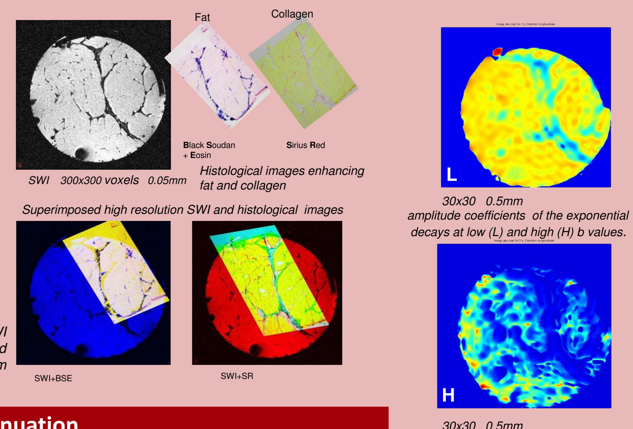
Comparison of high resolution SWI morphologic structural images and parametric diffusion images obtained from low resolution pulsed spin echo sequence.
