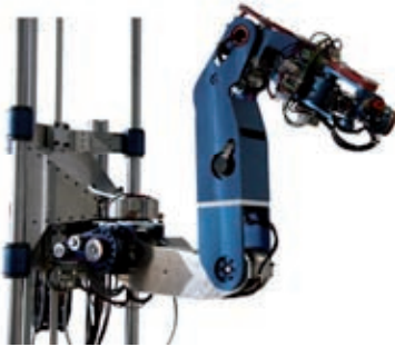
Fig. 6: Prototype of manipulator
