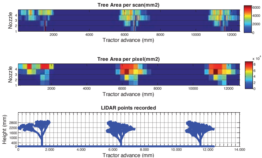
Figure 3. Scan (above), pixel (middle) tree area and LIDAR points detected (below)
