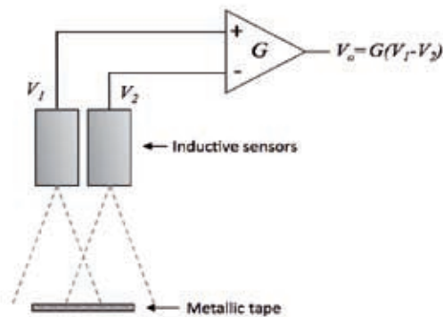
Fig. 2 – Schematic diagram of the tape tracking system based on a couple of proportional inductive sensors.
