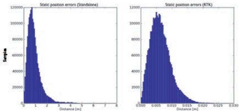
Fig.1. Static tests
