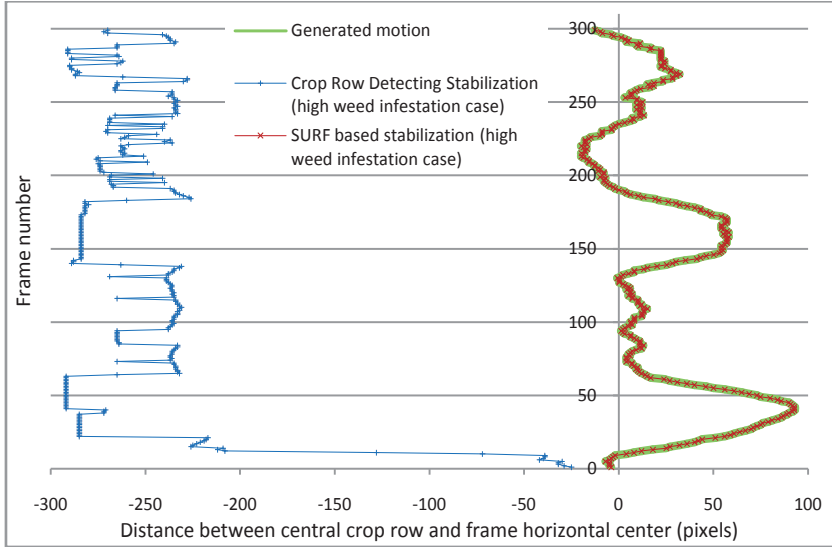
Fig. 2. Stabilization results for a field area where weed infestation is high. Only SURF based stabilization is successful.
