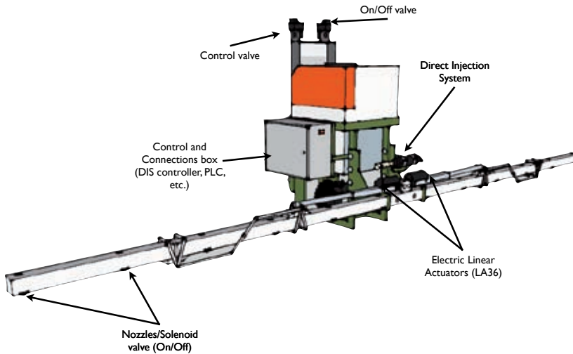
Fig. 1. Prototype weed control system built for initial tests
