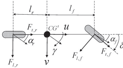
Fig. 1. Dynamics bicycle model for a tractor-implement system: velocities, side slip angles and forces at different locations of the system.
