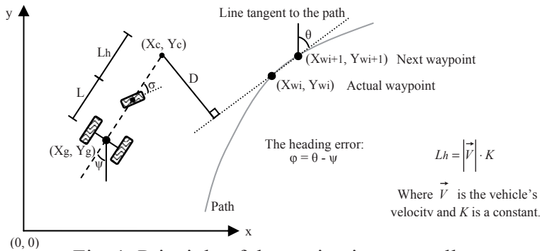
Fig. 1. Principle of the navigation controller.
