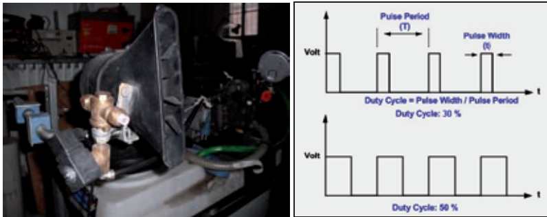
Fig. 1 - The solenoid valves to obtain a pulsed jet (left) and the HFSV operative scheme (right).
