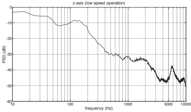
Fig.2. Power spectral density of vibration recorded on the direction of z-axis, low speed operation
