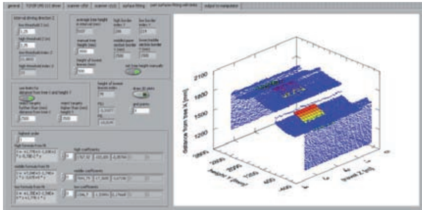
Fig. 3. Front panel of the laser scanner sensing module, stationary sprayer. Each surface corresponds to canopy surface.
