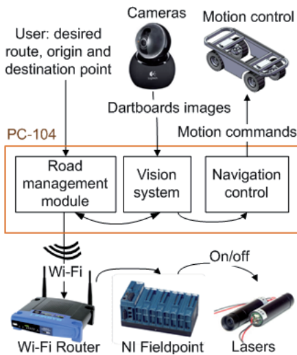
Figure 3. Architecture of the laser-based guiding system
