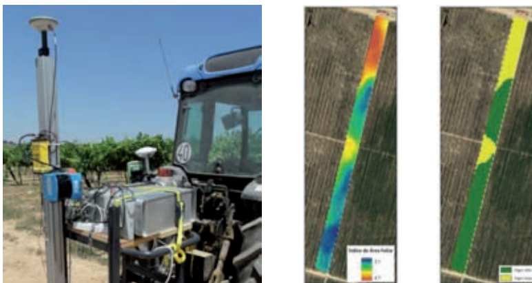
Fig. 1. LiDAR based system to scan canopy rows equipped with an RTK-DGPS receiver and an inertial unit (left) and the obtained LAI map (center) and vigour zones map (right).
