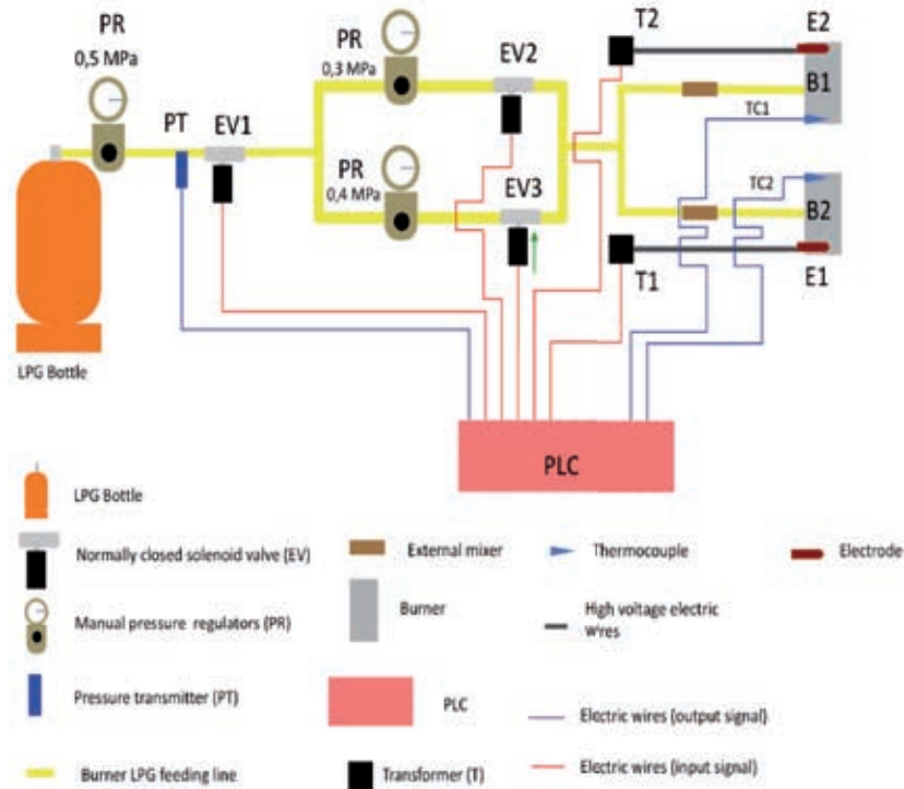
Fig. 1. Scheme of the LPG management system provided on the autonomous ground mobile unit: PR) manual pressure regulator; PT) pressure transmitter; EV1) normally closed solenoid main electro-valve; EV2-EV3) normally closed solenoid secondaries electro-valves; PR) pressure regulator; T) transformer; E) electrode; PLC) programmable logic controller.
