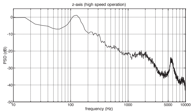
Fig.3. Power spectral density of vibration recorded on the direction of z-axis, high speed operation.
