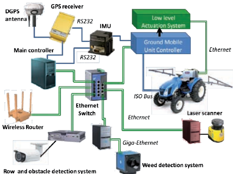
Fig. 1. General scheme of hardware architecture for an autonomous mobile robot for precision agriculture
