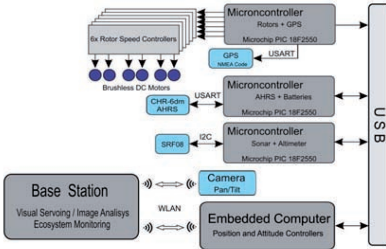
Fig.2. The hardware architecture
