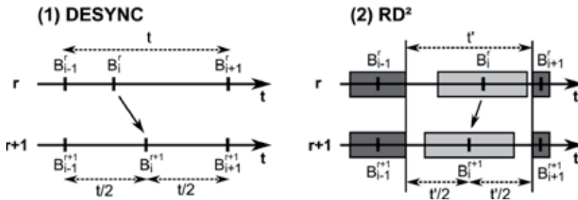
Fig. 1. Comparison between DESYNC and RD 2
