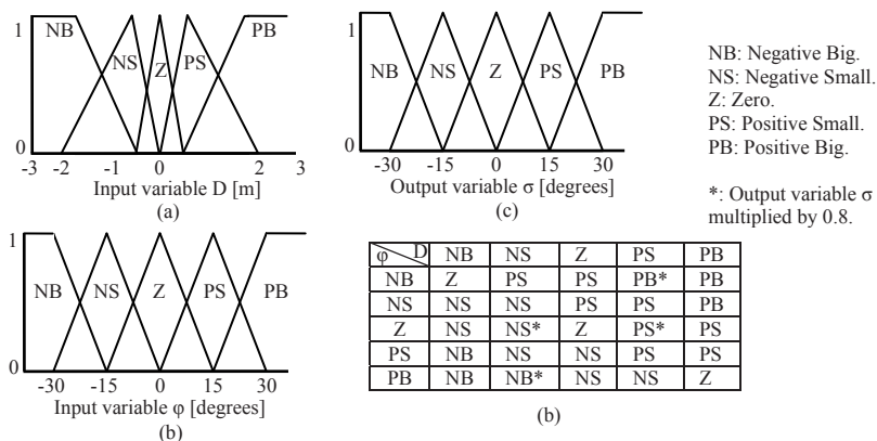
Fig. 2. Membership functions for: (a) lateral deviation; (b) heading error; (c) steering angle. (d) Base rule.
