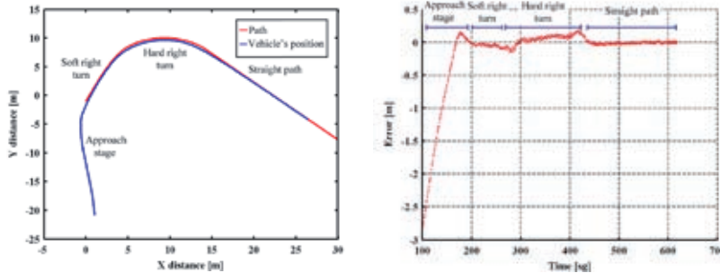
Fig. 4. Evaluation of the fuzzy logic positioning controller for lateral error correction. (Left) Position of the vehicle (blue) while following the user-defined path (red). (Right) Lateral error in the different stages of the path.
