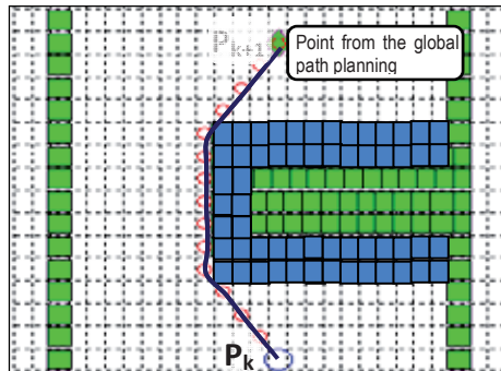
Fig. 3. Path for local obstacle avoidance and smoothing using cubic Bezier curves. ■ Offset of the obstacle.
