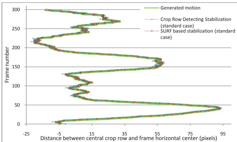
Fig. 1. Stabilization results for a standard field area where crop rows are easily identifiable. Both algorithms work properly.
