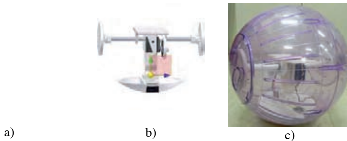
Figure 1: ROSPHERE v0.2. a) Concept. b) CAD design of inner mechanical system. c) Real prototype
