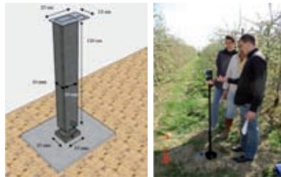
Fig. 1 : Metal support for the camera
