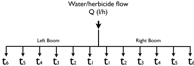
Fig. 2. Diagram of 12 solenoid valve/nozzles times
