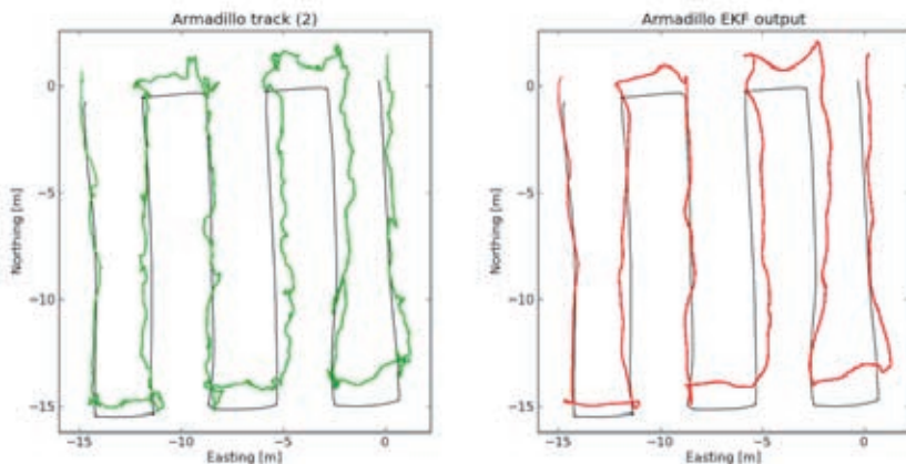
Fig.3. Armadillo track and EKF output
