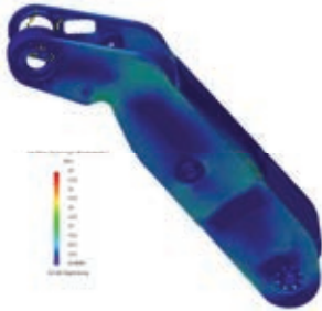
Fig. 4: Von Mises-Stresses of link 4
