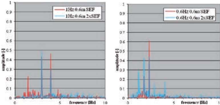
Fig. 5: Spectra of influence of distance and rotation speed on leaves displacements, left: screen rotation 1/s, right: screen rotation 0.6 /s.
