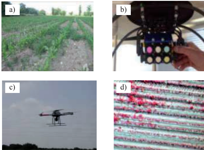
Fig. 1. a) Patches of grass weed seedlings ( Sorghum halepense ) in maize crop; b) 6-channel multispectral camera; c) UAV flying; d) aerial image (color-infrared composition) collected by the UAV at 30 m altitude, showing a sampling square frame (upper right corner in white).
