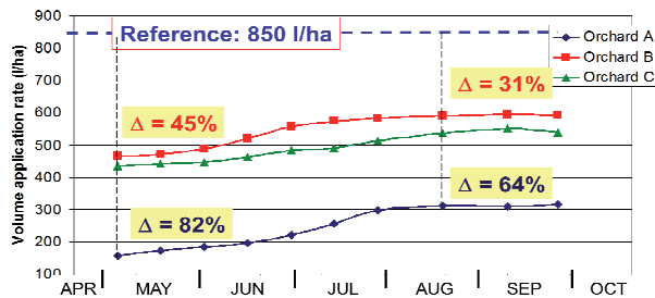
Fig. 3. Volume application rates used across the season with a sprayer controlled by Crop Identification System (variable rate application), calibrated for 850 l/ha as a reference volume, in three different orchards: (A) 2-year Gala cv., trees 2,2 m tall; (B) 11-year Red Chief cv., trees 4,0 m tall; (C) 13-year Gala cv., trees 4,0 m tall.
