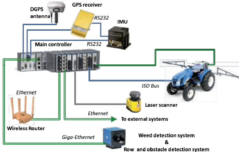
Fig. 2. Prospective hardware configuration for RHEA
