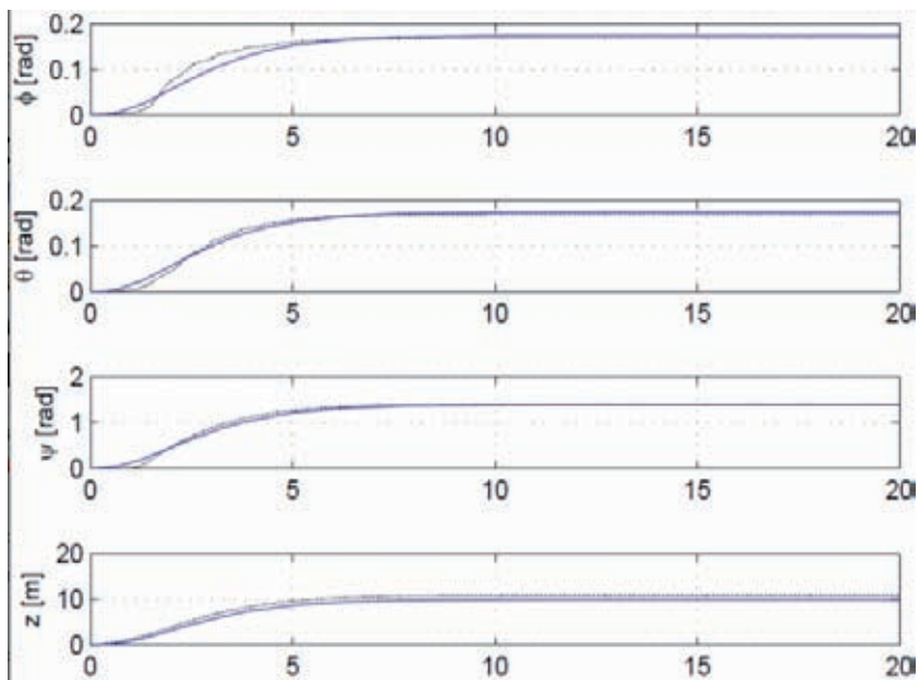
Fig. 3. Attitude and altitude of the helicopter.
