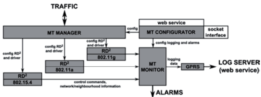
Fig. 2. Architecture of the RHEA communication system
