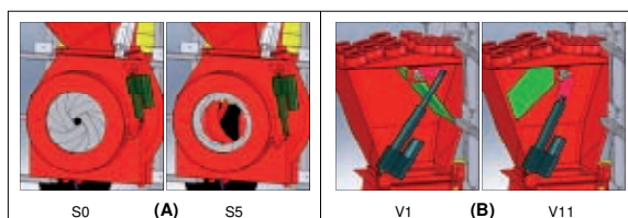
Fig. 2. Airflow adjustment device of the Environmentally Dependent Application System: (A) diaphragm leaf shutter on the inlet of radial fan (positions: S0 – closed; S5 - fully open); (B) air vane in the air collector (positions: V1 – no air to the right section and full air to the left section; V11 – no air to the left section and full air to the right section).
