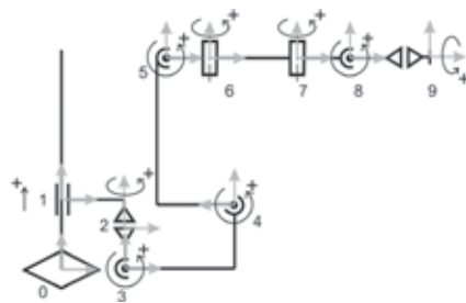
Fig. 2: Concept of the manipulator with nine degrees of freedom (DOF)
