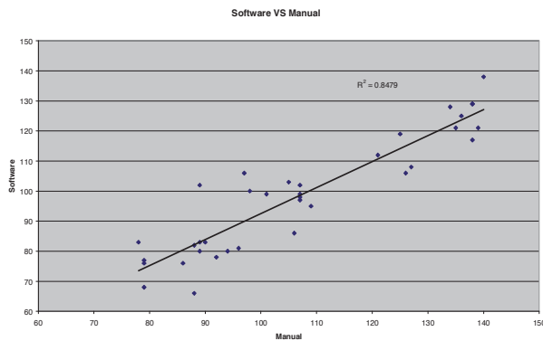
Fig. 7 : Manual count VS automatic
