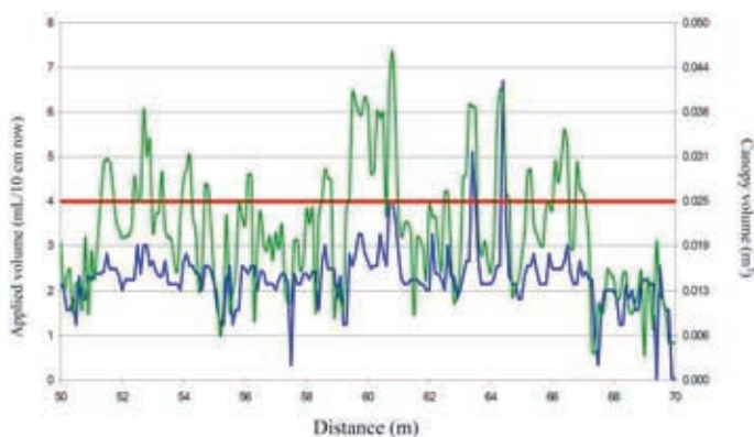
Fig. 3. Canopy volume (green line), variable rate sprayed volume (blue line) and constant flow rate application (red line) evolution along a vineyard row.
