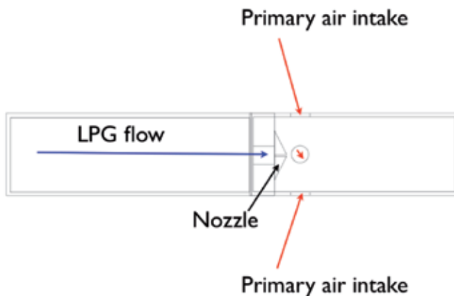
Fig. 2. Scheme of the LPG/Primary air external mixer.
