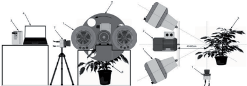
Fig. 2: Measurement setup: 1) SEF, 2) rotating airflow screen with four holes, driven by electric motor, 3) electric motor variable drive, 4) PC, 6) ficus plant, 7) high speed camera.
