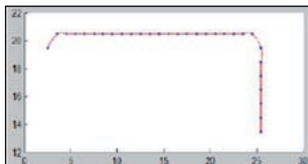
Fig.4. Smooth path using cubic Bezier curves, from Scenario 1.
