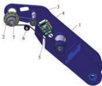
Fig. 3: Detailed assembly of element 4
