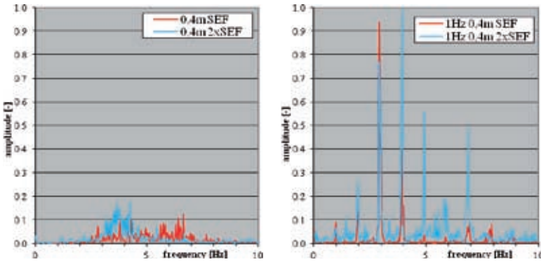
Fig. 4: Spectra of plant leaves displacements at distance 0.4 m, left: without excitation, right: with excitation, screen rotational frequency is 1 /s.
