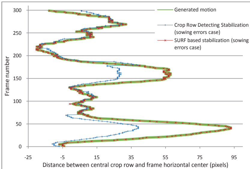
Fig. 3. Stabilization results for both algorithms in a problematic field region where there have been sowing errors.
