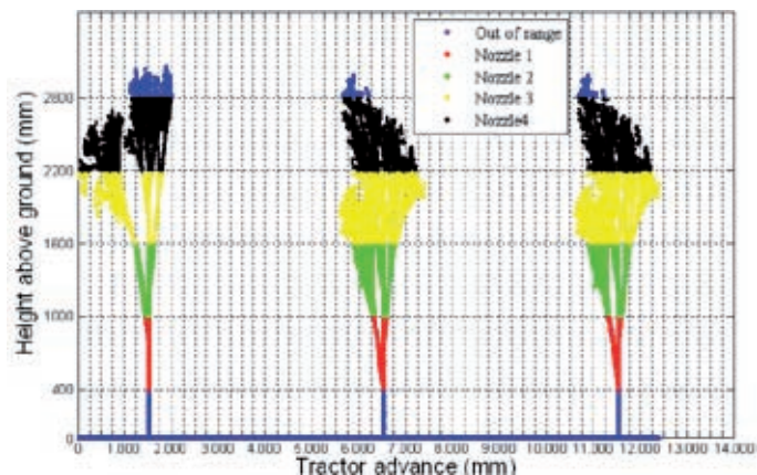
Figure 1. Minimum actuation areas (pixel) represented by different colors each spray nozzle.
