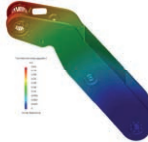
Fig. 5: Displacements of link 4
