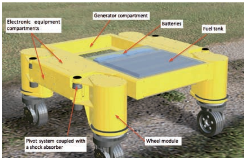
Fig. 1 – 3D rendering of the robotic platform basic structure
