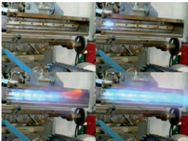
Fig. 3. Sequence of the electric ignition of the burner at the working pressures of 0.4 MPa.
