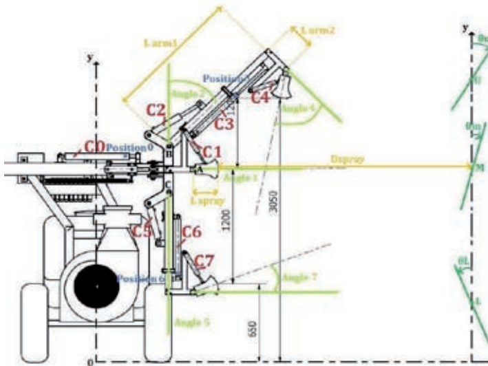
Fig. 2. Degrees of freedom of the spraying arm. Hydraulic cylinders (C0 to C7) represent degrees of freedom. Dark green lines are multidimensional surfaces fitted to the canopy.
