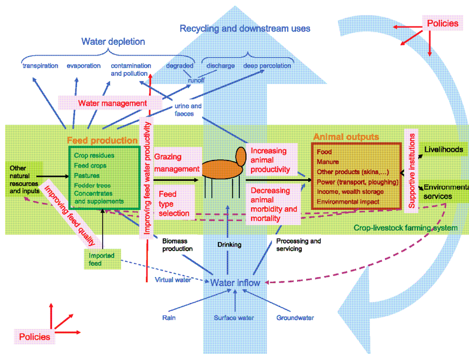
Figure 1. LWP framework
