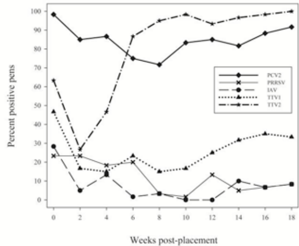
Figure 1. Percentage of pen oral samples testing positive via PCR.
