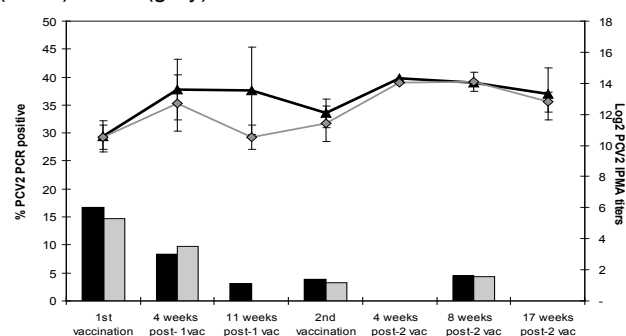
Figure 1: Percentage of PCV2 PCR positive serum samples (bars) and mean log 2 (±SD) PCV2 IPMA titres (lines) in A (black) and B (grey) sows.
