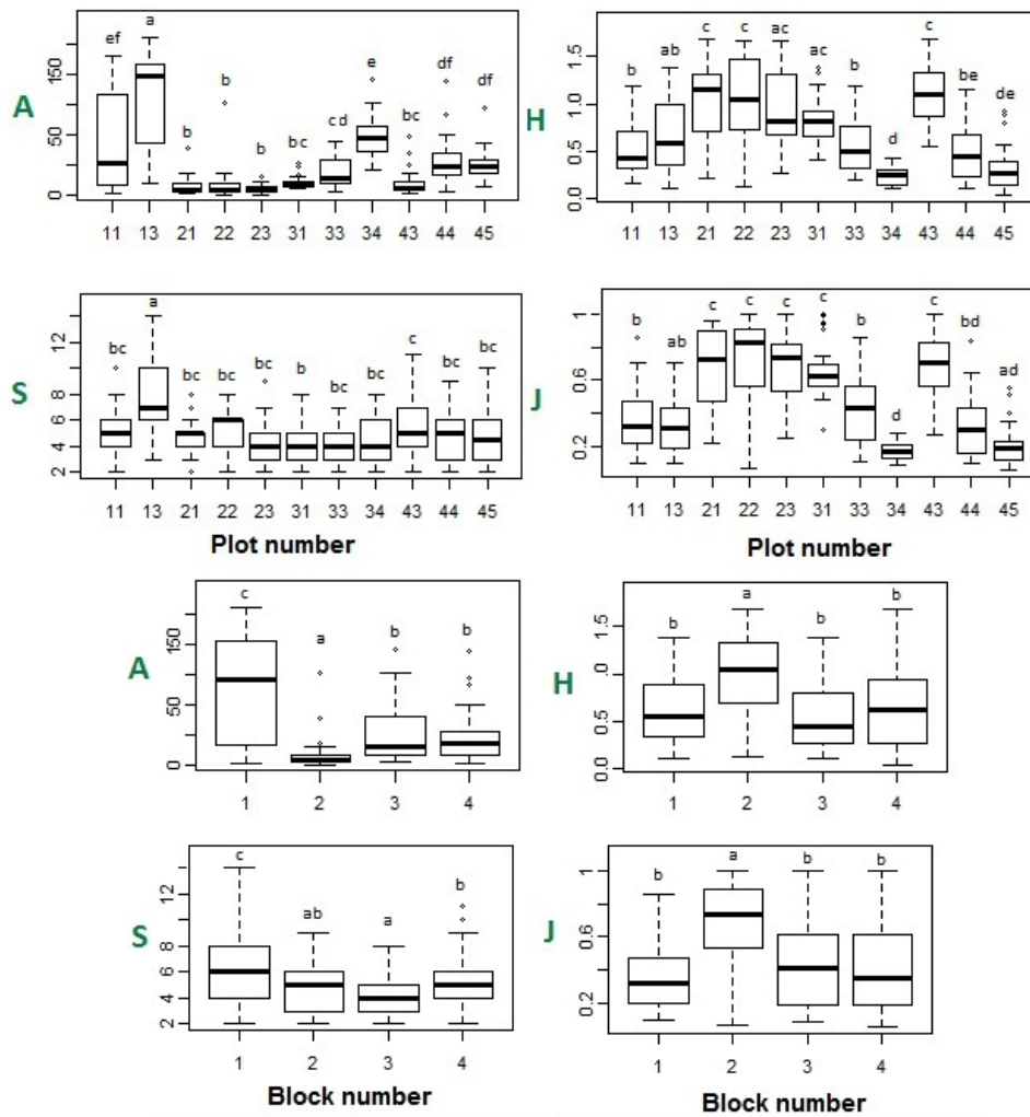
Figure 1 et 2 : Boxplots of total abundance of seed A (number of seed \times 10^3/m^2 ), specific richness index S, diversity Shannon index H and evenness Pielou index J of the seed bank (2005). The input data for boxplot were calculated per core of soil. Within each index boxplot, the same lowercase letters are not different at the 5% probability level. Abscise label at plot scale is composed of 2 numbers (XX), respectively the block and the plot.
