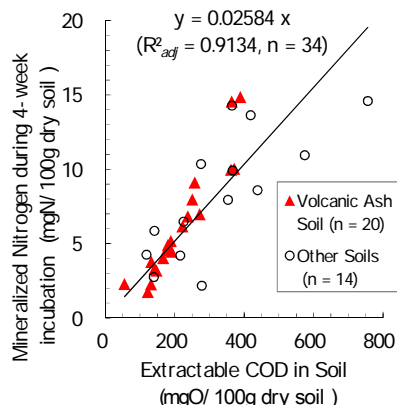
Figure 3. Relationship between available N and COD in soil.
