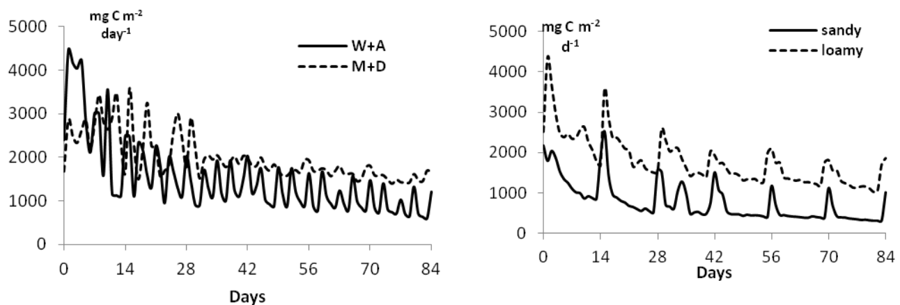
Figure 3a,b: C-CO 2 emission during decomposition of wheat+alfalfa mulch (W+A) and maize+dolichos mulch (M+D) on loamy soil (left) and comparison of sandy and loamy soil with decomposing M+D mulch (right). Peaks correspond to application of rain on columns.
