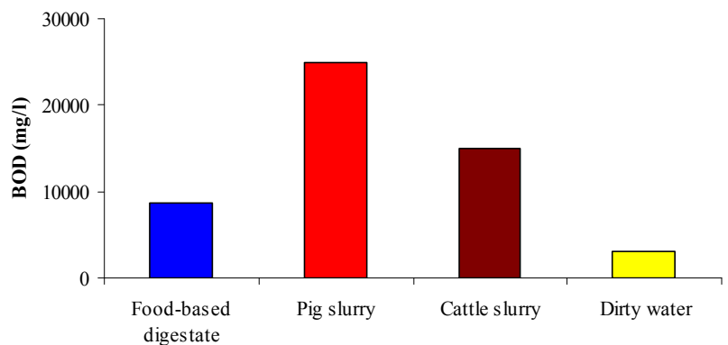
Figure 1. Biochemical oxygen demand (mg/l) of digestate, 'typical' pig and cattle slurries and dirty water (MAFF, 1998).
