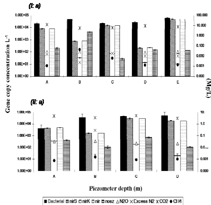
Figure 1. Mean groundwater nirK , nirS , nosZ and bacterial 16S rRNA GCC L -1 filtered at (OP I: a) spring barley, (Depth – A & B=5 m) (Depth – C & D=10 m); (Depth – E=20 m) (II: a) DG grazed clover ryegrass grassland.
