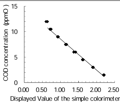
Figure 1. Measurement range of the proposed method for COD standards.
