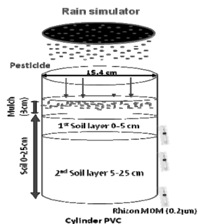
Figure 2. Experimental design for the soil columns
