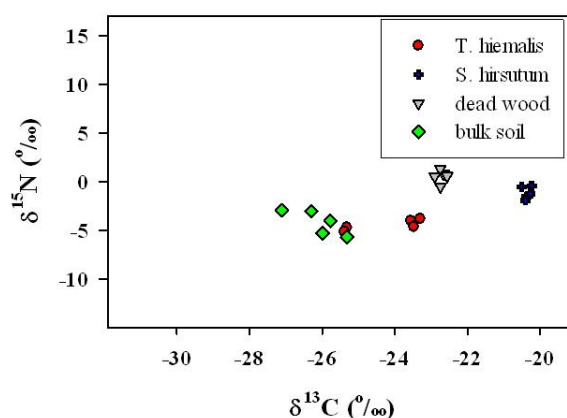
Figure 2: Discrimination among the two saprotrophic sporophores collected in the Châteauevert stand in 2003 according to \delta^{13}\text{C} and \delta^{15}\text{N} (all sporophores, average and standard deviation). Comparison with soil and wood \delta^{13}\text{C} and \delta^{15}\text{N} . Tubaria hiemalis lives on soil and Stereum hirsutum on wood. There is a statistically significant \delta^{13}\text{C} shift between soil and Tubaria hiemalis and between wood and Stereum hirsutum . There is no statistically significant \delta^{15}\text{N} shift between the two fungi and the two corresponding substrates.
