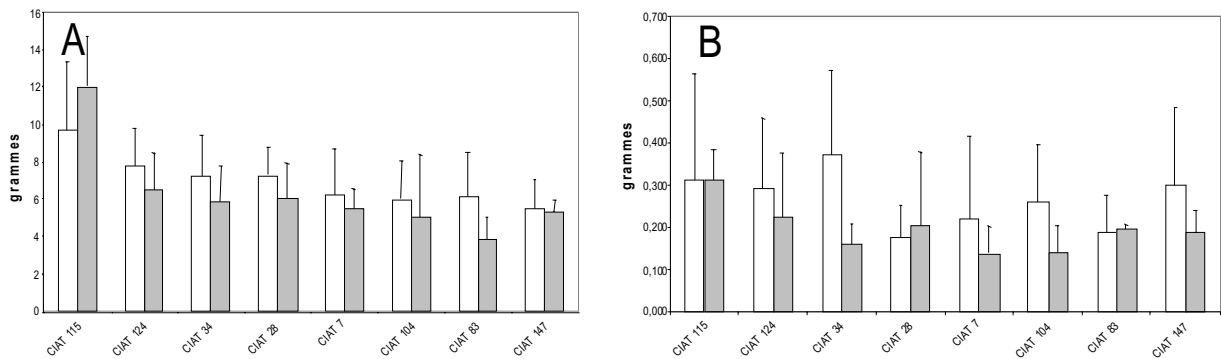
Fig. 2. Biomass of shoot (A) and nodules (B) of contrasting recombinant inbred lines of the cross of BAT477 x DOR364 in glasshouse hydroaeroponic culture under sufficient (white) versus deficient (grey) P supply. Data are means and standard deviation of 10 replicates at flowering stage
