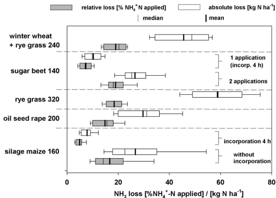
Figure 1. Simulated cumulated relative and absolute NH_3 losses 5 days after application of biogas residues, 1997-2008 ( n = 12 ), Hohenschulen, Germany; values = fertilizer N_{tot} [ kg\ ha^{-1} ], error bars = 5% - 95% quintile
