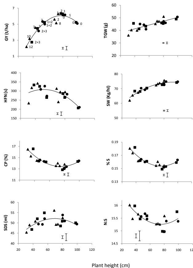
Fig. 1: Grain yield and quality against height (cm) of winter wheat in three varietal backgrounds (Mercia =triangles; Maris Huntsman = squares; M. Widgeon = circles). o = rht (tall); 1 = Rht-B1b; 2 = Rht-D1b; 3 = Rht-B1c; 8 = Rht8c+Ppd-D1a; 10 = Rht-D1b; 12 = Rht12). Error bars are min. and max. SEDs.
