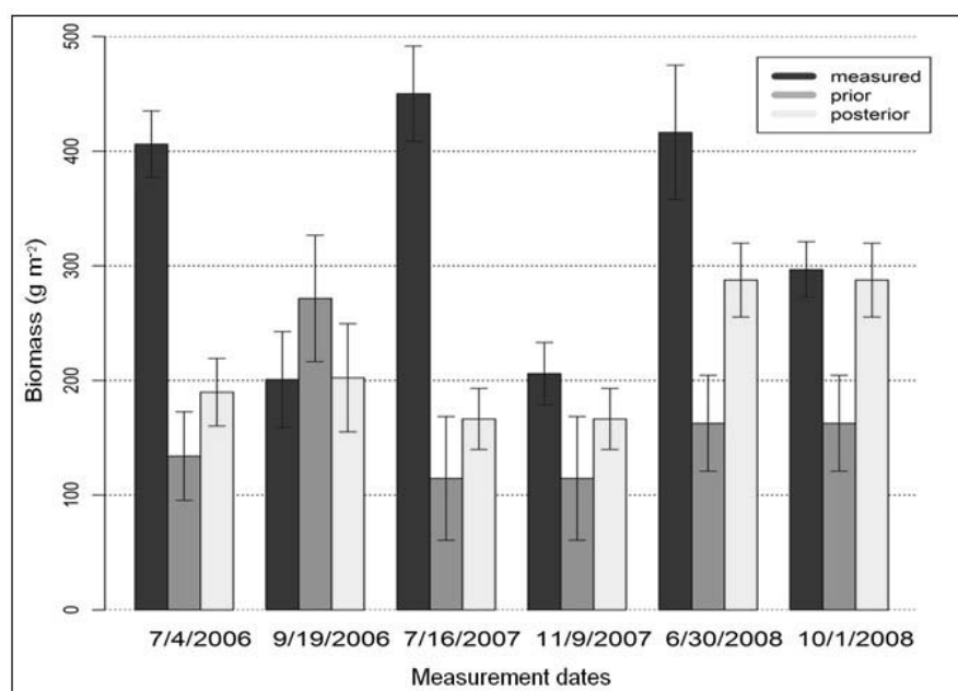
Figure 1. Uncertainty analysis for prior and posterior estimates of simulated biomass obtained at Früebüel for the treatment plots (vertical bars are standard deviations)
