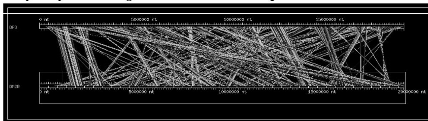
Fig. 2. Conservation of syntenic regions between human chr21 and mouse chr16. Lack of conservation between syntenic regions of D. melanogaster chr2R and D. pseodobscura chr3. In the top figure a chromosomal region of human chromosome 21 is aligned with a chromosomal region of mouse chromosome 16. Lines have been drawn to link orthologous genes between these two regions. The majority of the lines are parallel to each other demonstrating in that way that the order of the orthologous genes has been conserved. On the other hand, for the comparison of the syntenic areas of chromosome 2R of D. melanogaster and chromosome 3 of D. pseodobscura we note that the order of the orthologous genes is not well conserved as the lines linking them are interconnected.
