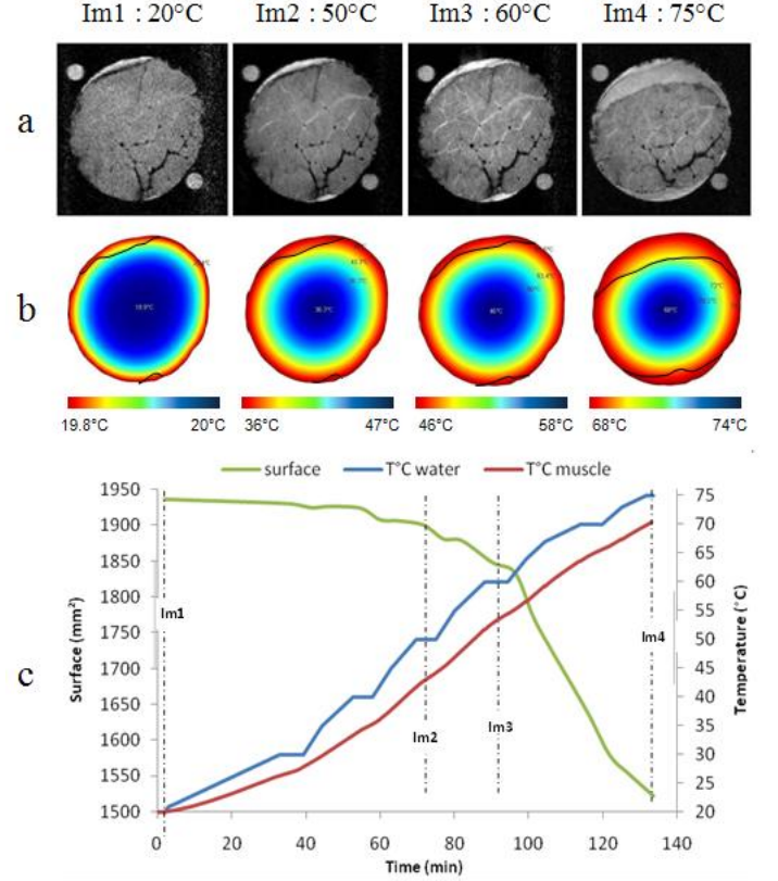
Fig.3. (a) NMR deformation images of a core section at different temperatures of the heating water, (b) images simulating corresponding temperature gradients, (c) time course plots of the surface area of the muscle core section, the temperature of the heating water and the mean muscle temperature.
