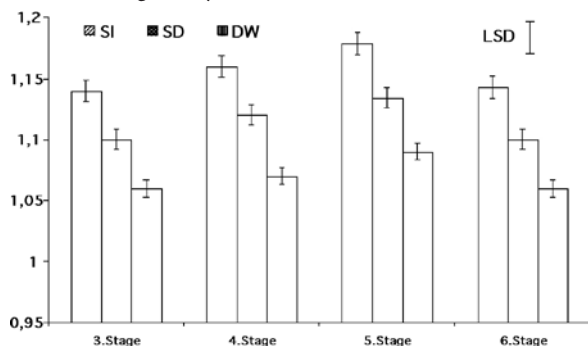
Fig.3. Effect of different growth media on \text{Chl}_{a+b} content of H_3 , H_4 , H_5 and H_6 of seedling for cotton cultivar ( \text{mg}\cdot\text{g}^{-1} fresh leaf weight). Symbols and abbreviations correspond to those in Fig.1.
