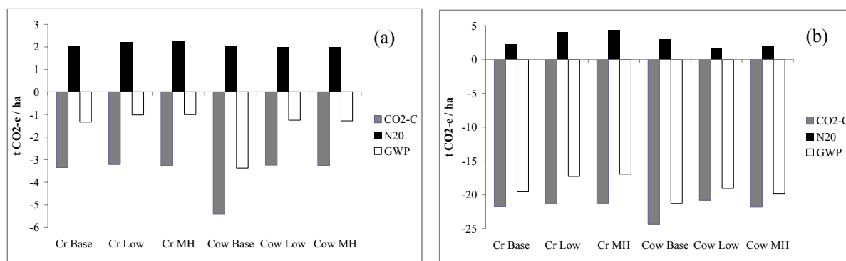
Figure 1. Carbon sequestration, N 2 O and global warming potential for the (a) fertilizer treatment and (b) slurry treatment for Crichton (Cr) and Cowpark (Cow) weather conditions for current (Base), and the low (Low) and medium-high (MH) UKCIP02 emission scenarios.
