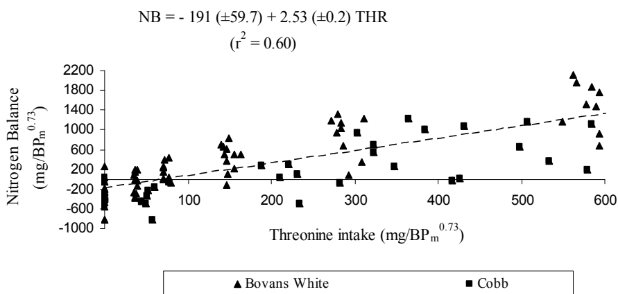
Figure 1. Regression of nitrogen balance on daily threonine intake ( \text{mg/BP}_m^{0.73} ), to determine the Thr for maintenance.
