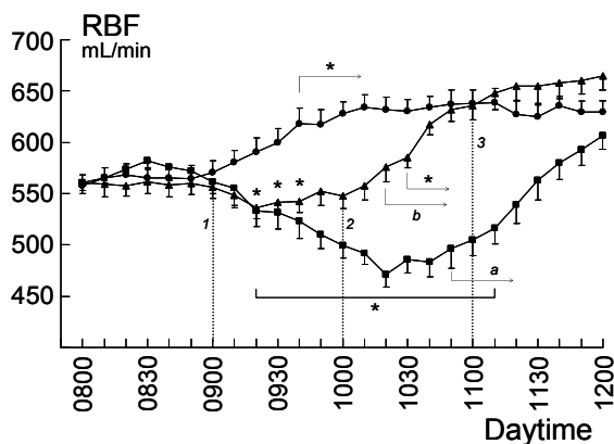
Figure 1. Renal blood flow (RBF) during and after 2 h perfusions of mixed AA (●, dotted lines 1-3) and of L-NAME (■) and ketoprofen (▲) (dotted lines 1-3) with mixed AA during the second hour (dotted lines 2-3). Data are 10 min means \pm SE. * = P < 0.05 vs. 1 h pre-infusion mean value; a, b = P < 0.05 vs. the minimum value in L-NAME (1020) and ketoprofen (0920) perfusions; n = 6 sheep.
