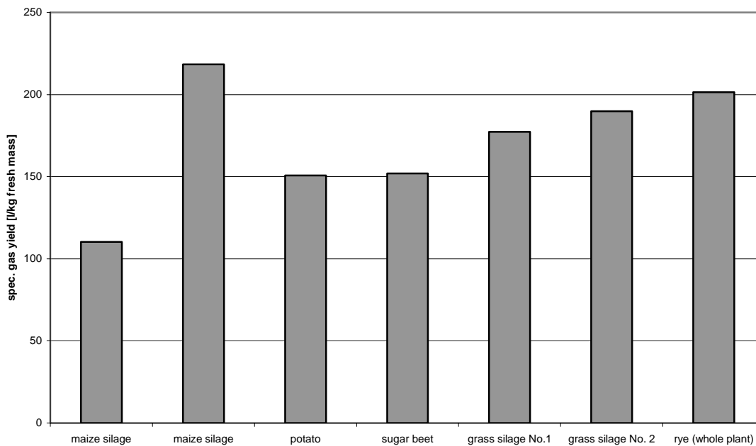
Figure 1: Specific fermentation gas yields of individual substrates (HASSELMANN 2006, p. 53)
