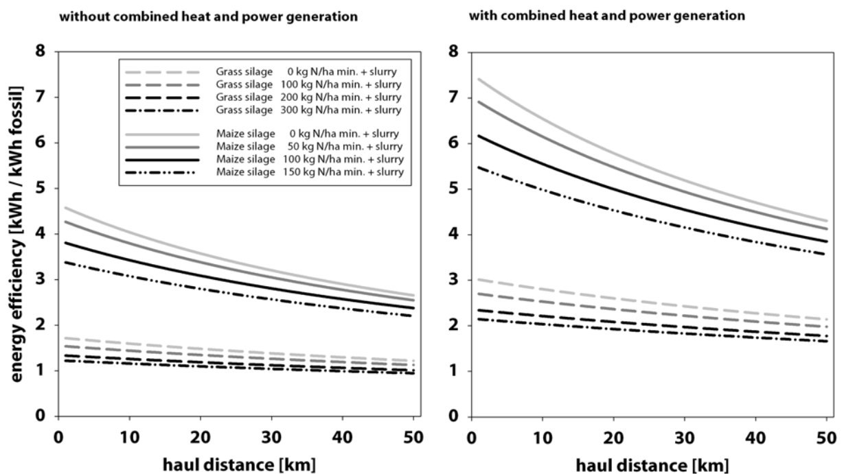
Figure 1. Energy efficiency (units energy produced per unit fossil energy input) of biogas production from grass silage and maize silage with/without power-heat coupling, depending on the distance between field and fermenter and N fertilisation (data source: N-project Karkendamm, grassland with 4 cuts versus maize monoculture).
