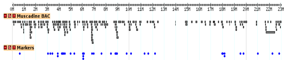
Figure 1. Snapshot of a view on the genome browser showing the alignment of the M. rotundifolia BACs on chromosome 1 of the grapevine reference genome.
