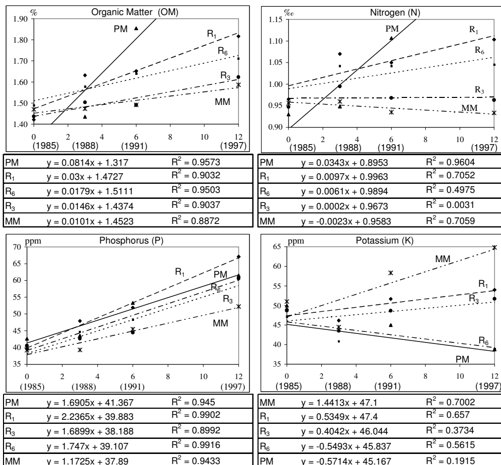
Figure 2. OM, N, P and K variations in the soil after 12 years
