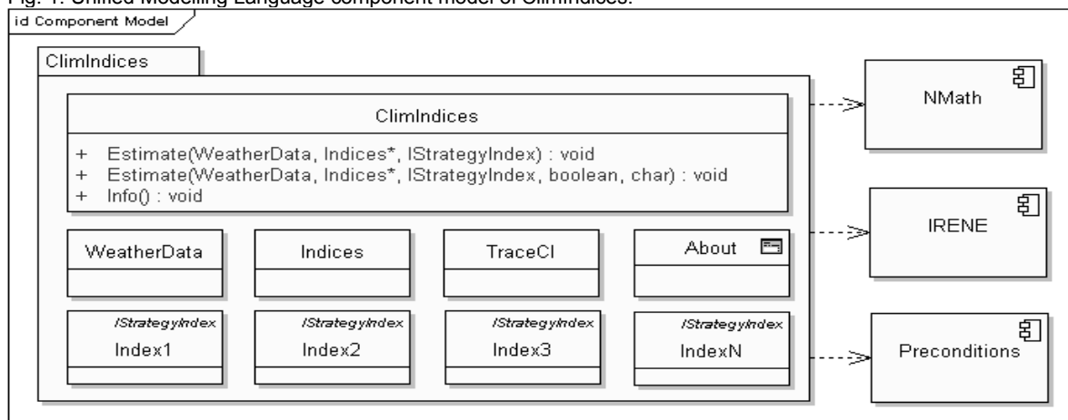
Fig. 1. Unified Modelling Language component model of ClimIndices.
