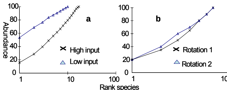
Fig 1. K dominace test, Abundance Plots.
