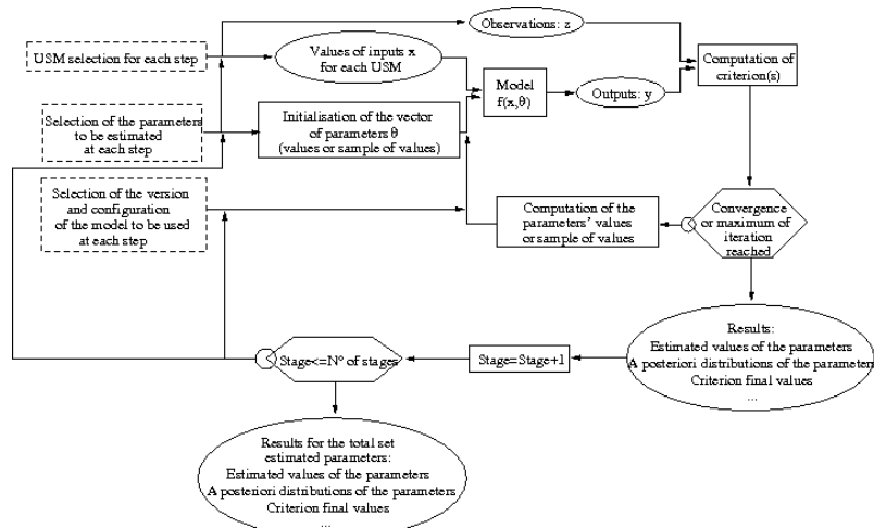
Figure 1. Algorithm diagram of iterative process.
