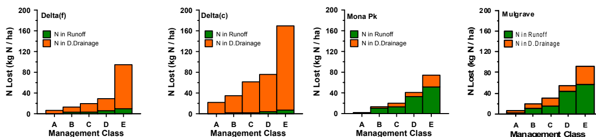
Figure 1. Predicted long-term annual losses of N via runoff and deep drainage at the four sites under five classes of management practices designed to meet water quality targets.
