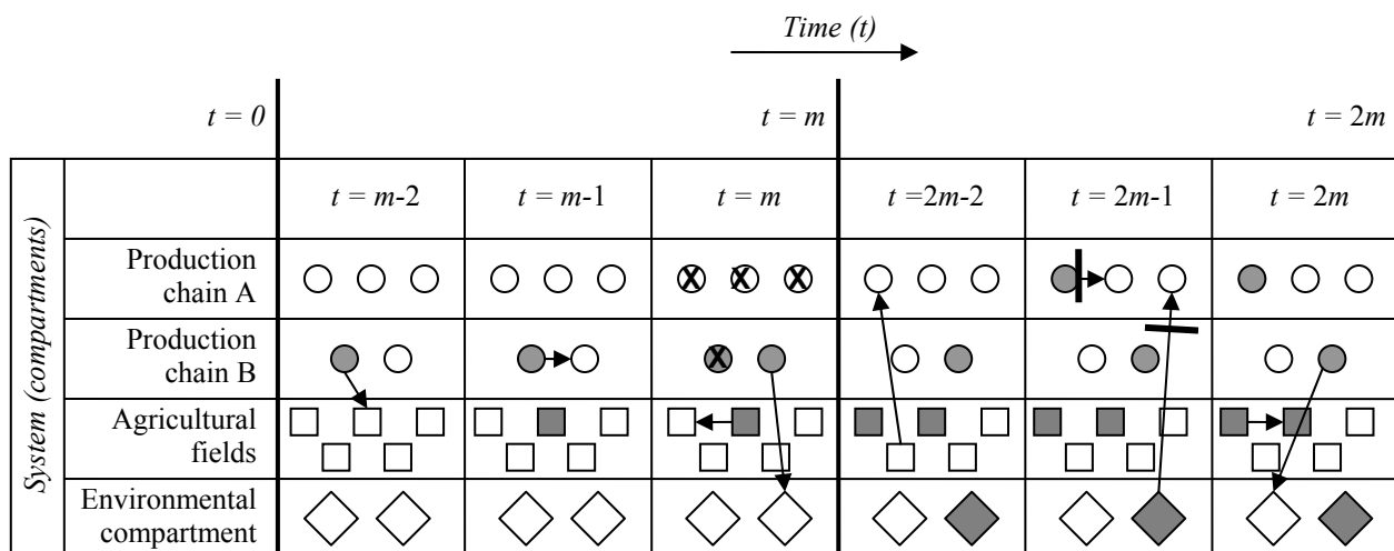
Figure 1. Schematic representation of modelled system according to the generic framework. Figures represent objects; shaded ones are infested. Arrows indicate transmission between objects; a bar indicates that transmission is blocked by a control measure. Objects with a cross are removed from the compartment.
