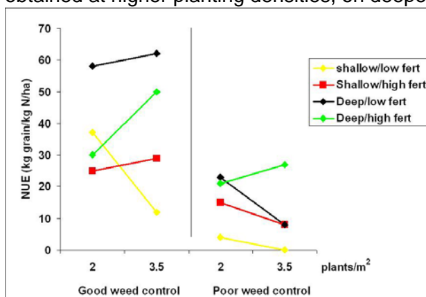
Figure 1a. Simulated nitrogen use efficiency (NUE) of fertilizer N at two densities of maize grown in shallow or deep soils with high and low fertility and poor and good weed control.
