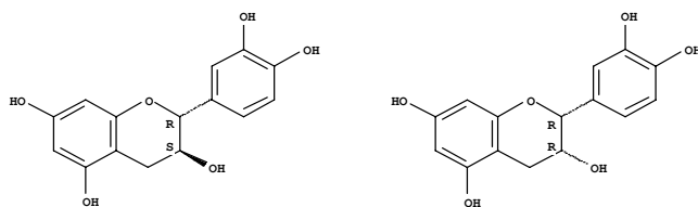
Figure: Chemical structures (absolute stereochemistry) of catechin (left) and epicatechin (right)
