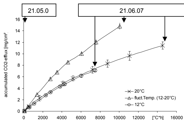
Fig. 1: accumulated \text{CO}_2 -efflux of 'Liberto' tomatoes in different postharvest temperature regime as a function of temperature impact.
