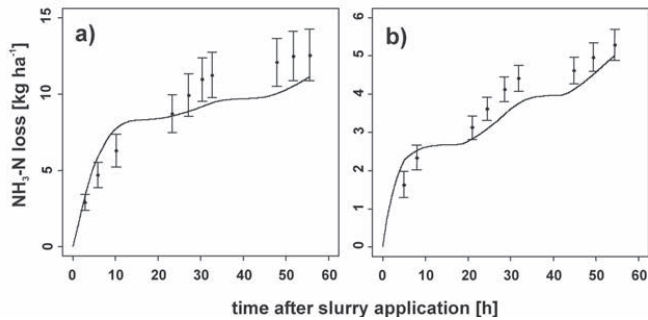
Figure 1: Measured \text{NH}_3 loss dynamics from biogas slurries applied to grassland sites (sandy soil) with trail hoses and simulated by the mechanistic approach (Eq. 1) for two parameterization data sets a) May 2007, 60 \text{ kg ha}^{-1} \text{ N}_{\text{tot}} b) May 2008, 120 \text{ kg ha}^{-1} \text{ N}_{\text{tot}} ; error bars = std. error ( n = 4 ), \text{N}_{\text{tot}} = mineral nitrogen + organic nitrogen in slurry
