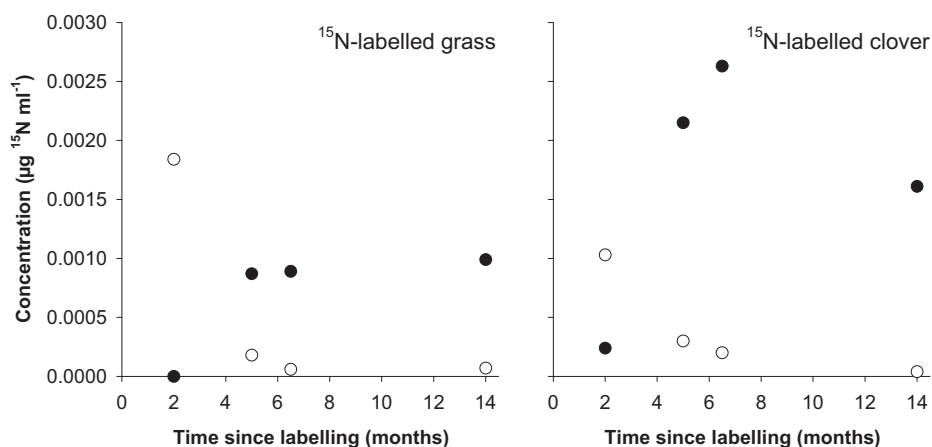
Figure 1. ^{15}\text{N} in DIN ( \circ ) and DON ( \bullet ) from leaf-labelled grass and clover at the December 2008 soil water sampling in Denmark as related to the time since labelling. The number of replicates on each data point varies from 1 to 3.
