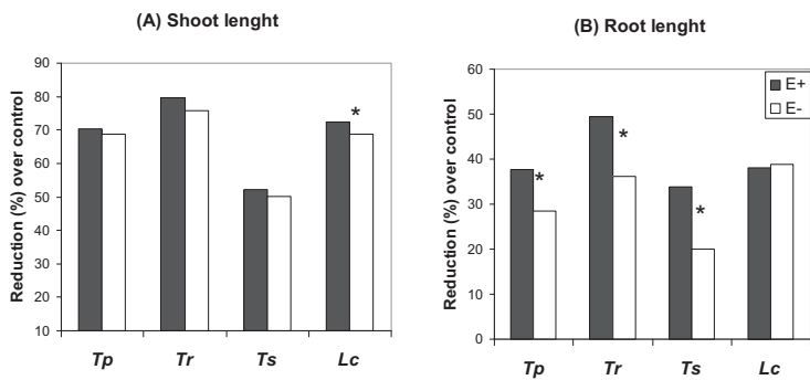
Figure 1. Reduction in shoot (A) and root (B) length (% over control) of four legume species ( Tp = T. pratense ; Tr = T. repens ; Ts = T. subterraneum ; Lc = L. corniculatus ) when growing with F. rubra plants infected (E+) and non-infected (E-) by the endophyte E. festucae . * = significant differences between E+ and E- pair of means at P < 0.05 ( n=20 ).
