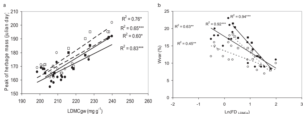
Figure 2. Date at which herbage peak occurred (a) and indicator of the growth curve shape (Wvar) (b) according to LDMCgw and \text{Ln}(\text{FD}_{\text{LDMCg}} \times 100) in 2002 (■, □) and in 2004 (●, ○) for whole herbage (full symbol) or the grass component (empty symbol); LDMCgw is leaf dry matter content weighted by the grass species abundance; FD is a functional diversity index established on LDMC basis; Wvar is the percentage of herbage mass 20 days before the peak in relation to peak; * P < 0.05 ; ** P < 0.001 ; *** P < 0.001
