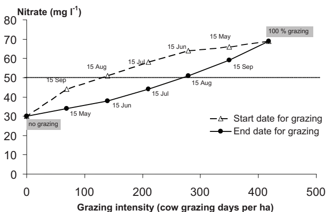
Figure 2. The effect of the length of the grazing season on \text{NO}_3 leaching. The upper line represents the starting dates of the grazing season, while the lower line represents the end dates of the grazing season. The modeled dairy farm has 80 cows, with a milk production of 8000 \text{ kg cow}^{-1} , on 35 ha of grassland on sandy soil, fertilised with 250 \text{ kg ha}^{-1} \text{ N} .
