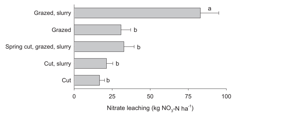
Figure 3. Nitrate leaching from grass-clover pastures with different management. In grazed grass-clover slurry was injected in the spring (100 kg ha -1 cattle slurry total-N), in cut-only grass-clover an additional injection of slurry was made following a spring harvest of herbage. Bars with the same letter indicate no significant difference ( P >0.05)
