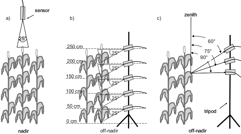
Figure 1: Schematic measuring setup for nadir (a) and off-nadir (b+c) measurements, including sensor field of view (a+b); segment heights (b) and zenith view angle (c)
