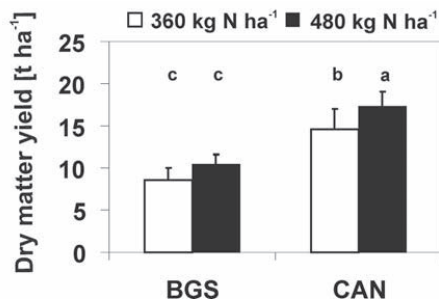
Figure 2 Dry matter yield [ \text{t ha}^{-1} ] of perennial ryegrass, cut 4 times a year, at a moderate ( 360 \text{ kg ha}^{-1} \text{ N} ) and a high level ( 480 \text{ kg ha}^{-1} ) of N fertilization with biogas slurry (BGS) and mineral fertilizer (CAN) in the marsh region of Schleswig-Holstein. Values with different letters are statistically different at P < 0.05 (Tukey-test, n=4 ).
