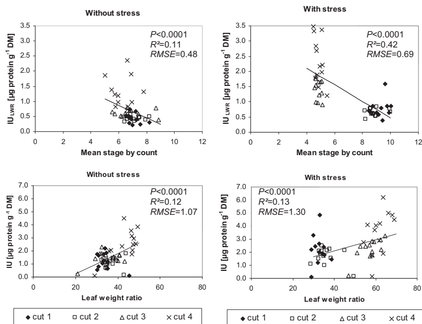
Figure 1: Relation between the specific PPO-activity and MSC or LWR of red clover genotypes. IU: Specific PPO-activity in IU (µg protein per g DM); IU LWR : Specific PPO-activity in IU related to LWR
