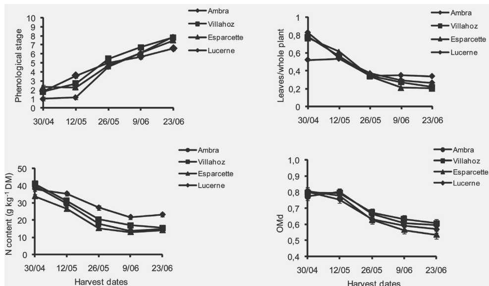
Figure 1. Time-course evolution of phenological stage (1=early vegetative, 2=mid vegetative, 3=late vegetative, 4=early bud, 5=late bud, 6=early flower, 7=late flower, 8=early seed pod), leaf to-whole plant ratio, N content in DM (g kg -1 ) and organic matter digestibility (OMd) at the different harvest dates, with standard errors.
