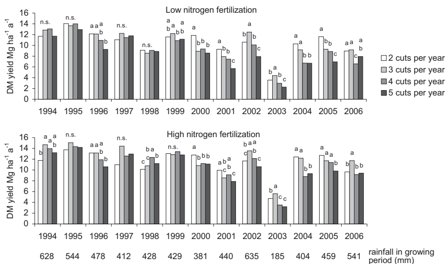
Figure 1. Annual dry matter (DM) yield and rainfall during the (re-)growth period. Different letters indicate significant differences between treatments ( P < 0.05 ), n.s. not significant.
