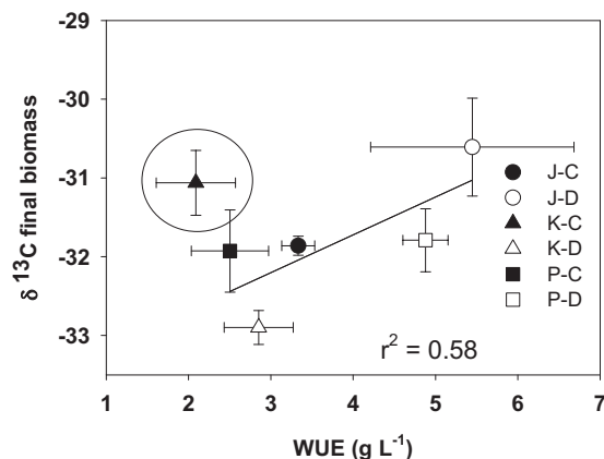
Figure 1. Relationship between isotopic composition of ^{13}\text{C} ( \delta^{13}\text{C} , ‰) in leaf final dry biomass and plant water use efficiency (WUE) (produced total biomass (g) / consumed water (L)). Values are means of 4 replicates \pm standard error. First letter refers to cv: J: Jana, K: Kasbah, P: Porto. Second letter refers to irrigation treatment: C: control, D: drought. The encircled point is out of the regression.
