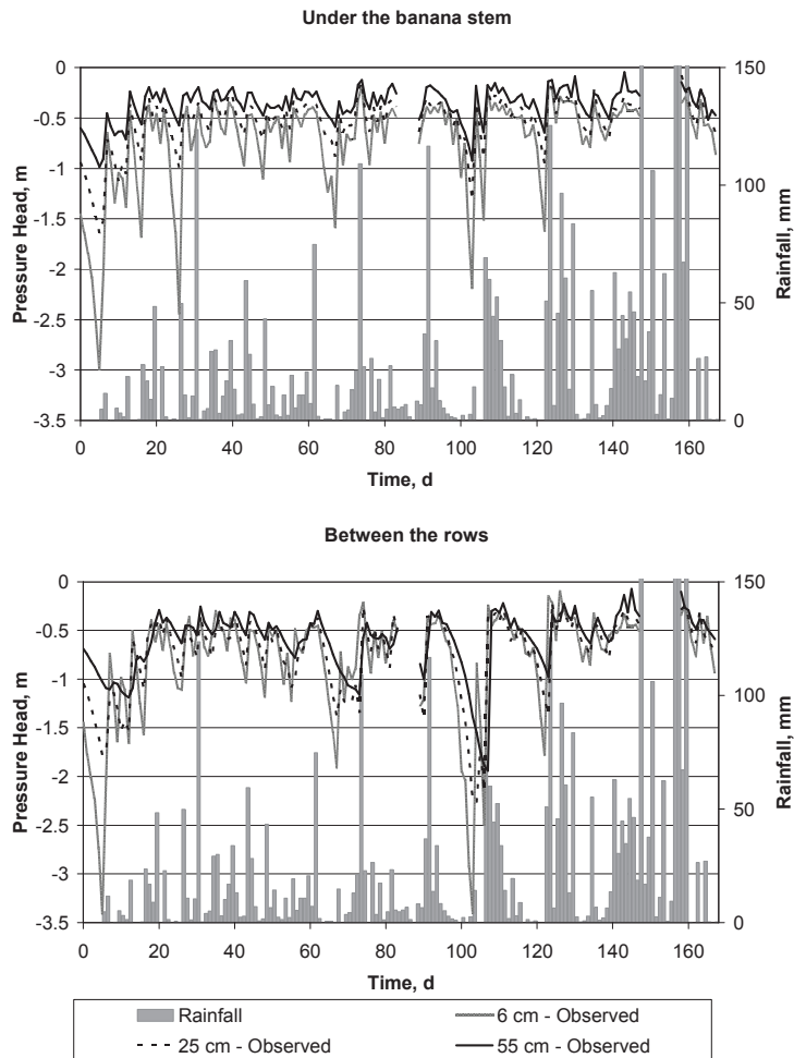
Fig. 4. Mean pressure heads (calculated from five sets, CV = 17%) measured with tensiometers in the soil (top) at the foot of the plant stem (Lysimeter 2) and (bottom) between rows (Lysimeter 4). Precipitation rates are also shown in both figures.
