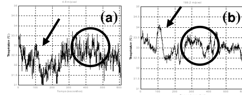
Figure 1. T s temporal evolution above a maritime pine stand over a 600s period at 1 Hz for 5 m (a), and 200 m (b) resolutions. Low frequency fluctuations related to convection in the PBL (arrow) are present regardless of the considered spatial resolution, whereas high frequency fluctuations are smoothed by spatial integration at pixel scale. The Y axis ranges between 31 and 35°C (after Lagouarde et al., 1997).
