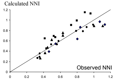
Fig. 3 : Comparison between observed and calculated NNI evaluated directly from CHL_{La} .
