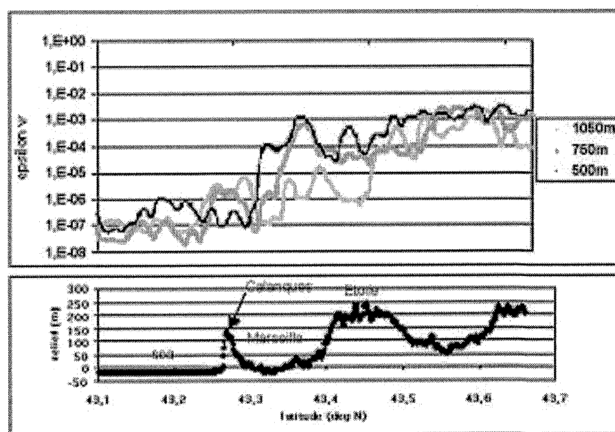
Figure 3. Dissipation rate of turbulent kinetic energy ( \text{m}^2\text{s}^{-3} ) measured with the Merlin IV (MeteoFrance) along the south-north legs at levels 1050, 750 and 500 m. The overflow relief is also represented with the sea on the left (south). The duration of the flight over the town, between the Calanques ridge to the south and the Etoile massif to the north, is 3 minutes. The energy spectrum high frequency tail is a relevant indicator of turbulence intensity in such inhomogeneous conditions.
