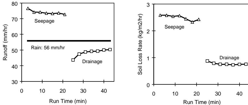
Figure 2. Changes in runoff and erosion as the Test Box was changed from seepage to drainage conditions during the rainstorm.
