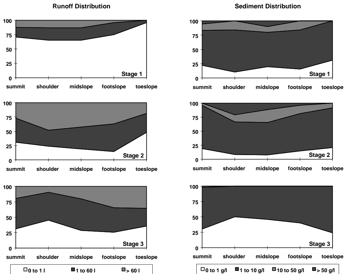
Figure 1. Partition of runoff and sediment at five hillslope positions from natural runoff plots.
