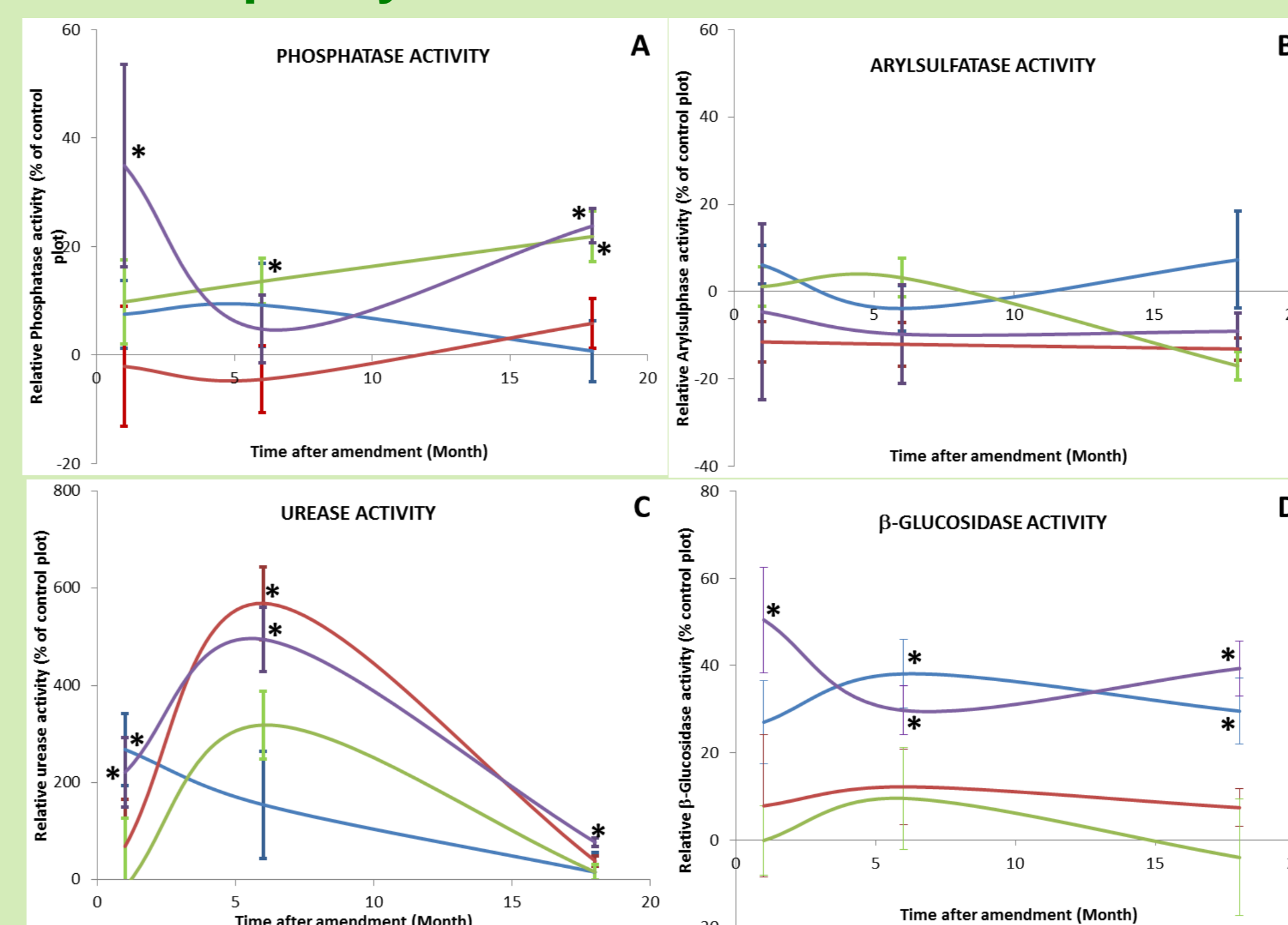
Time-course of hydrolase activities (expressed in % of control plot)
