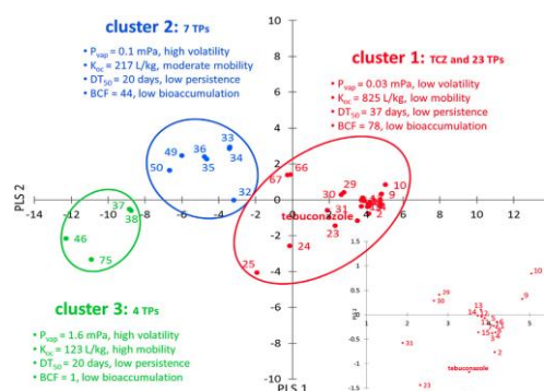
Figure 1. Categorization of TCZ and its 34 TPs into three clusters according to their molecular descriptors on the two main components of the PLS regression (PLS 1 and PLS 2), and their estimated environmental parameters (Storck et al., 2016).
