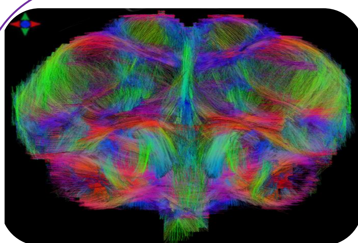
Connectogram
