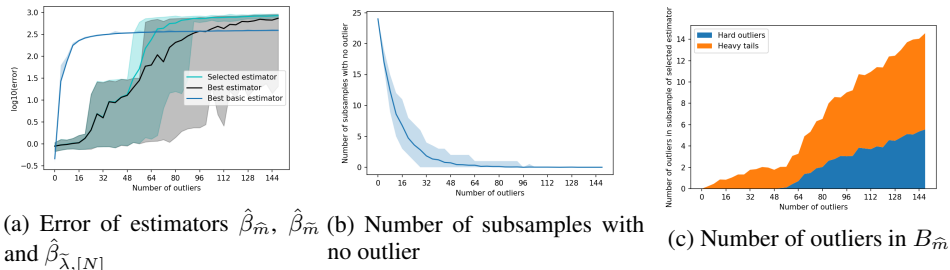
Figure 1: ensemble method run with N = 1000 , V = 40 , K_{\max} = 4 , and averaged over 200 experiments.
