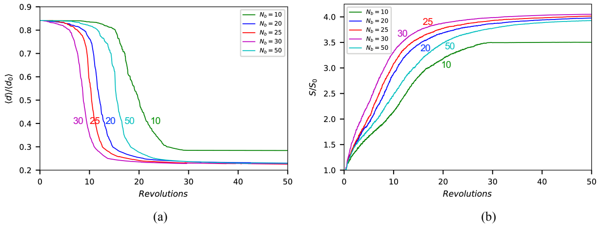
Figure 8. Evolution with the number of revolutions of a) normalized mean particle size and b) normalized specific surface, for different numbers of balls ( N_b ). The ball size D_b and the powder volume V_p are constant. Each curve consists of 1000 data points.
