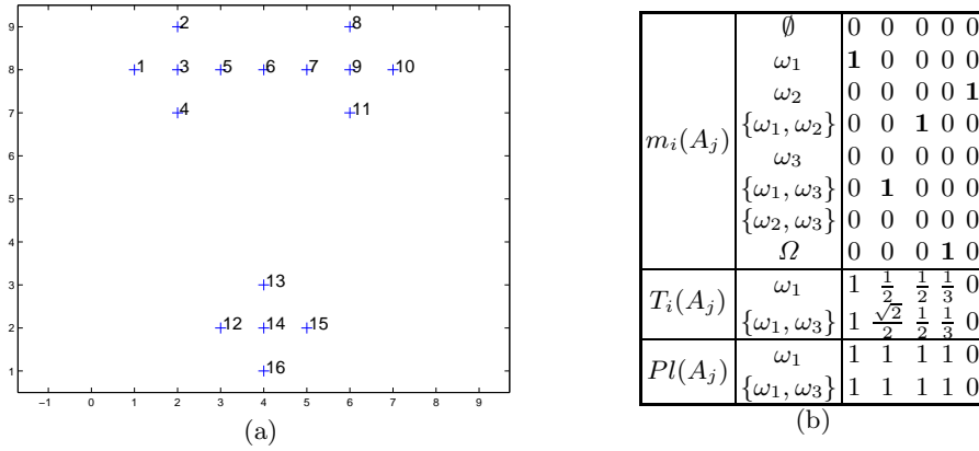
Fig. 1. DiamondK3 dataset (a) and illustration of the proposed penalty term T_i(A_j) when considering several possible mass functions and compared to penalty term based on plausibility Pl(A_j) for previous SECM-pl [7] (b).
