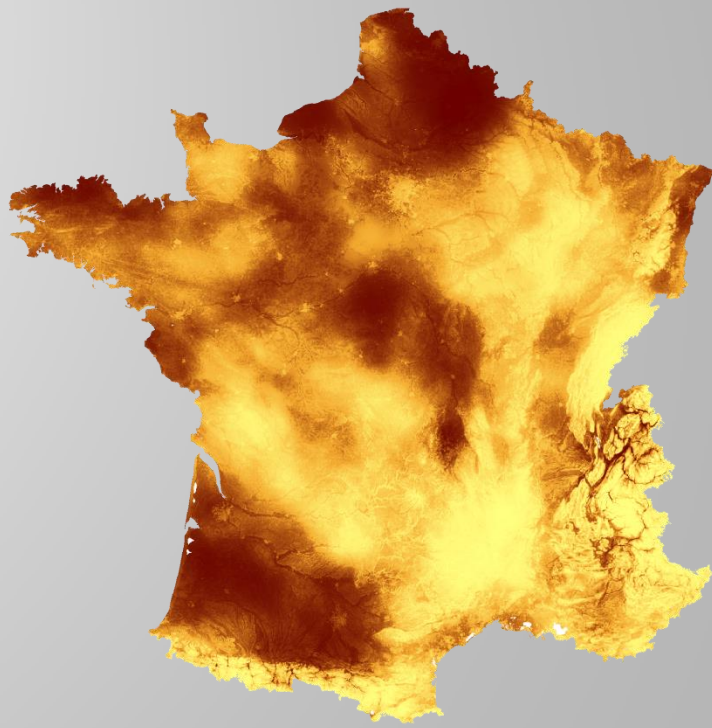
Multi-resolution kriging
