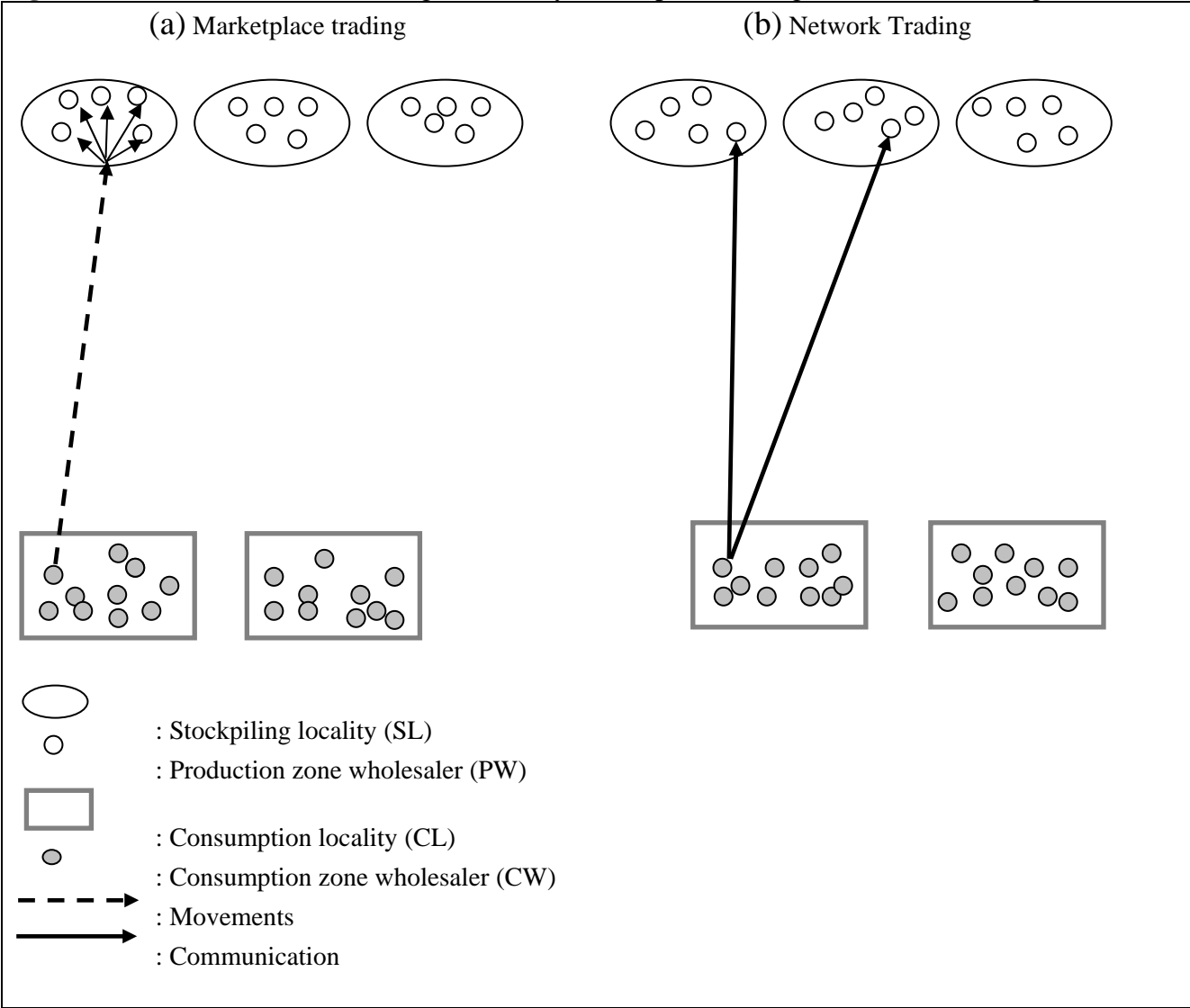
Figure 1. Communication channels generated by marketplace trading and network trading
