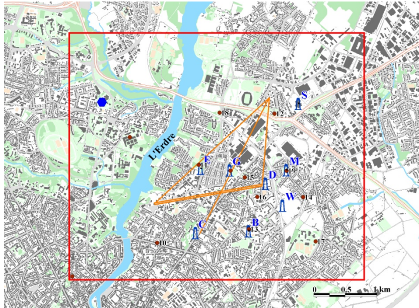
Figure 2. Measurement domain and set-up during the 2010 campaign: red dots, T-RH sensors; blue symbols, turbulent flux sensors on masts; orange lines, scintillometer paths; blue hexagon, Sodas; red frame, limits of the geographical data base.
