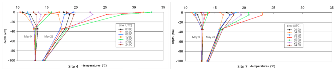
Figure 4. Temperature profiles in the ground at two sites.
